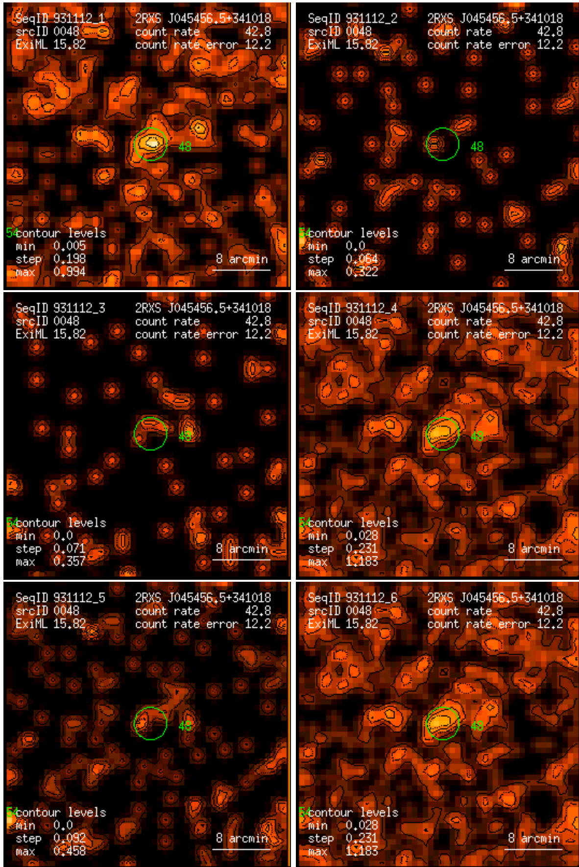
Figure 48: RASS 931112: detection 0048: band rate images, Gaussian filter: (1) PSPC channels 11 – 41, (2) 52 – 90, (3) 91 – 201, (4) 11 – 235, (5) 52 – 201, (6) 11 – 201. Broad band rates in counts/ks. Band rate contour levels in counts/ks/arcmin 2 .
