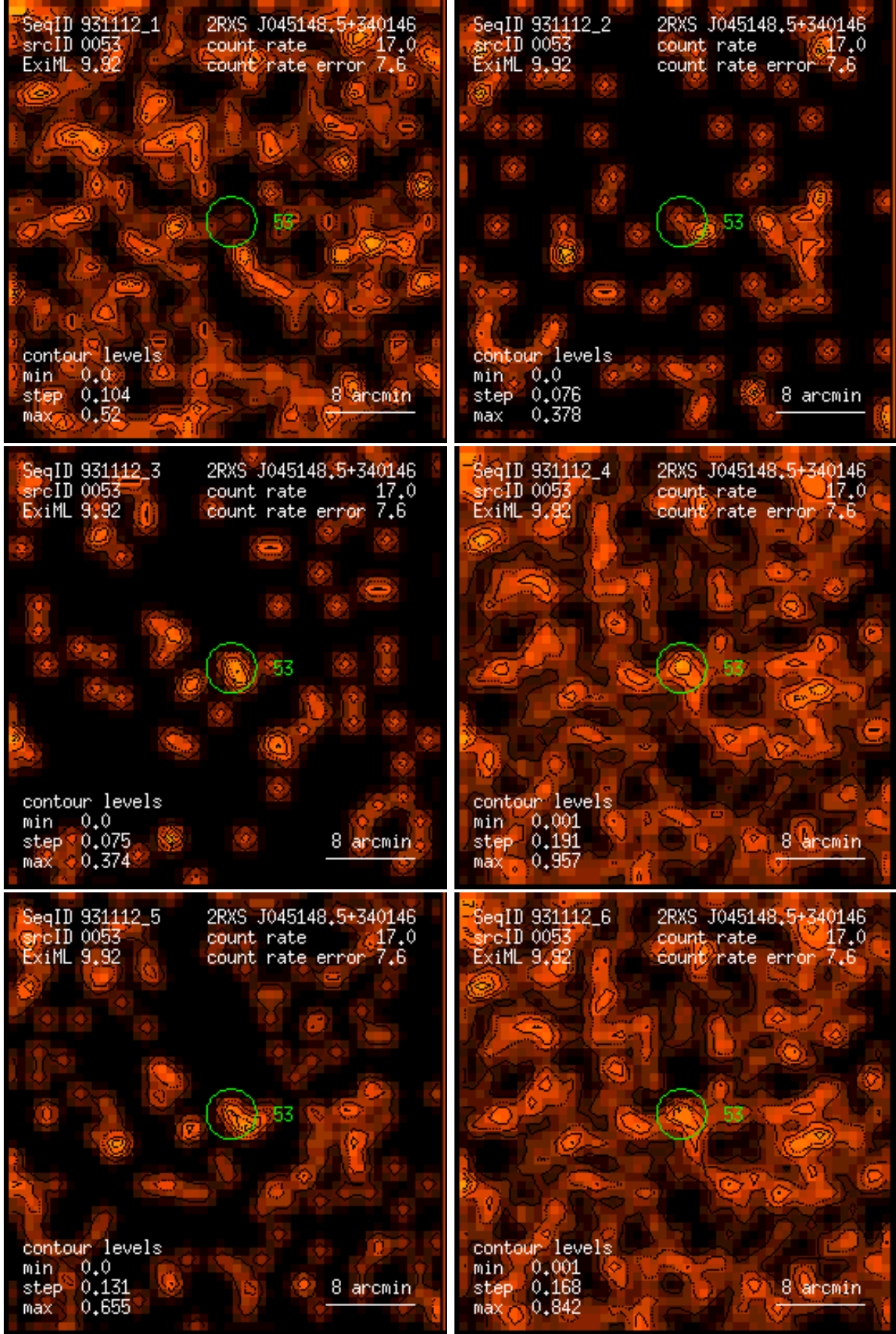
Figure 53: RASS 931112: detection 0053: band rate images, Gaussian filter: (1) PSPC channels 11 – 41, (2) 52 – 90, (3) 91 – 201, (4) 11 – 235, (5) 52 – 201, (6) 11 – 201. Broad band rates in counts/ks. Band rate contour levels in counts/ks/arcmin 2 .
