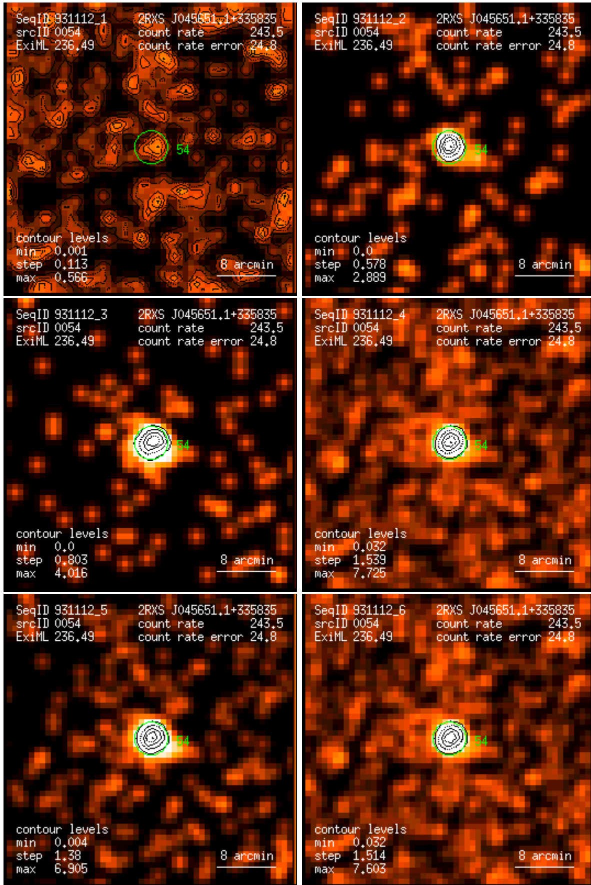
Figure 54: RASS 931112: detection 0054: band rate images, Gaussian filter: (1) PSPC channels 11 – 41, (2) 52 – 90, (3) 91 – 201, (4) 11 – 235, (5) 52 – 201, (6) 11 – 201. Broad band rates in counts/ks. Band rate contour levels in counts/ks/arcmin 2 .
