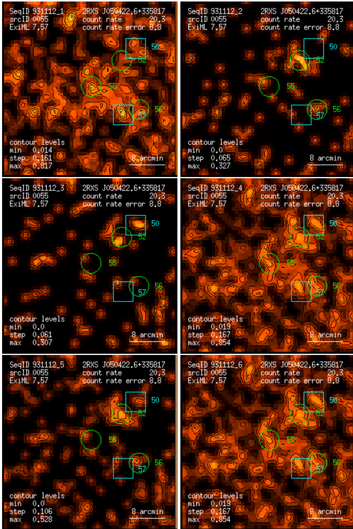
Figure 55: RASS 931112: detection 0055: band rate images, Gaussian filter: (1) PSPC channels 11 – 41, (2) 52 – 90, (3) 91 – 201, (4) 11 – 235, (5) 52 – 201, (6) 11 – 201. Broad band rates in counts/ks. Band rate contour levels in counts/ks/arcmin 2 .
