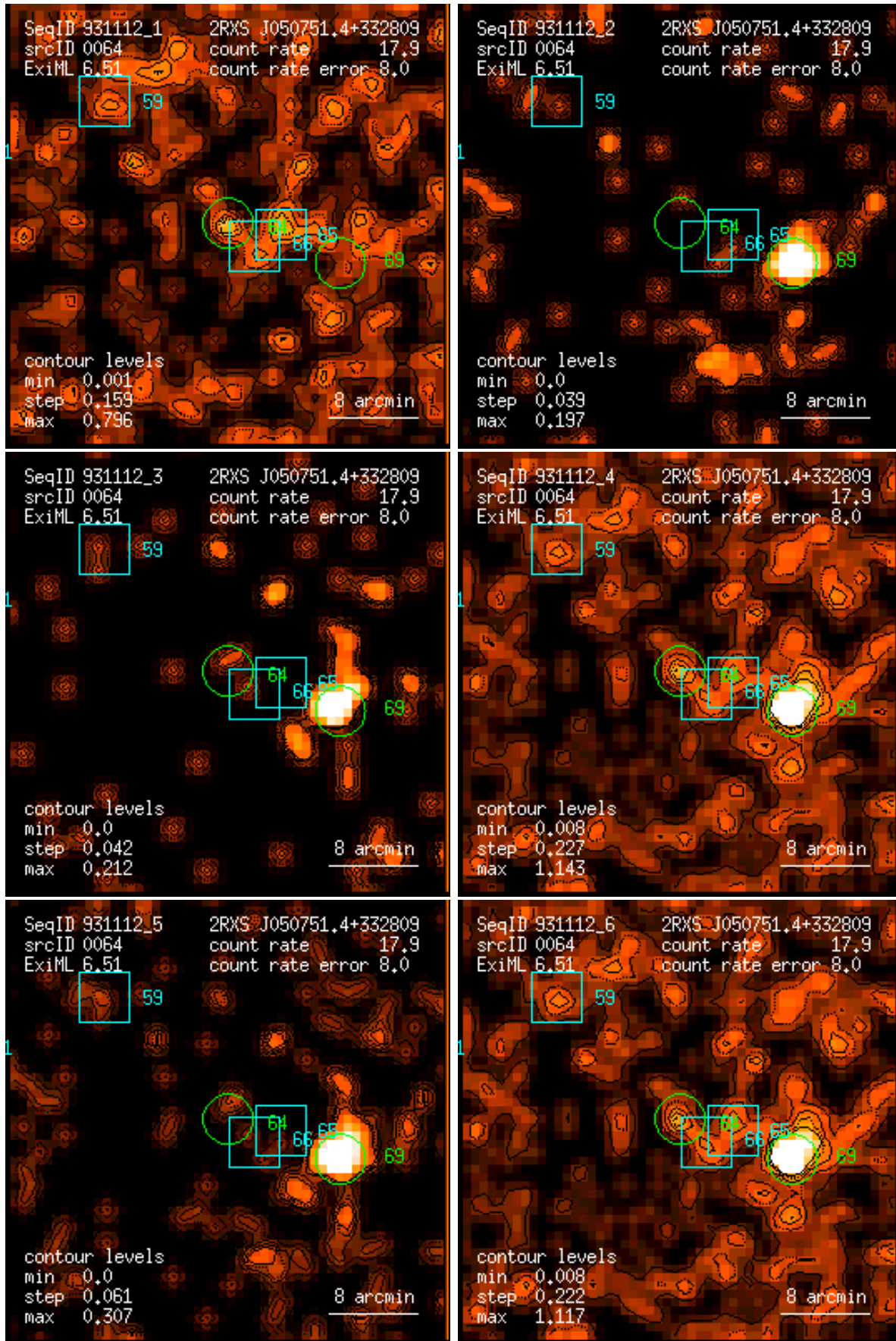
Figure 64: RASS 931112: detection 0064: band rate images, Gaussian filter: (1) PSPC channels 11 – 41, (2) 52 – 90, (3) 91 – 201, (4) 11 – 235, (5) 52 – 201, (6) 11 – 201. Broad band rates in counts/ks. Band rate contour levels in counts/ks/arcmin 2 .
