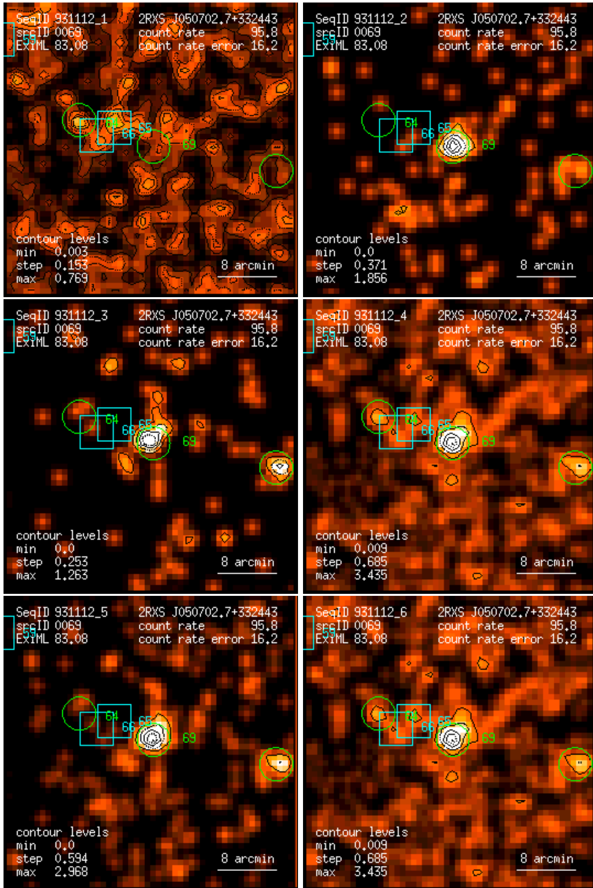
Figure 69: RASS 931112: detection 0069: band rate images, Gaussian filter: (1) PSPC channels 11 – 41, (2) 52 – 90, (3) 91 – 201, (4) 11 – 235, (5) 52 – 201, (6) 11 – 201. Broad band rates in counts/ks. Band rate contour levels in counts/ks/arcmin 2 .
