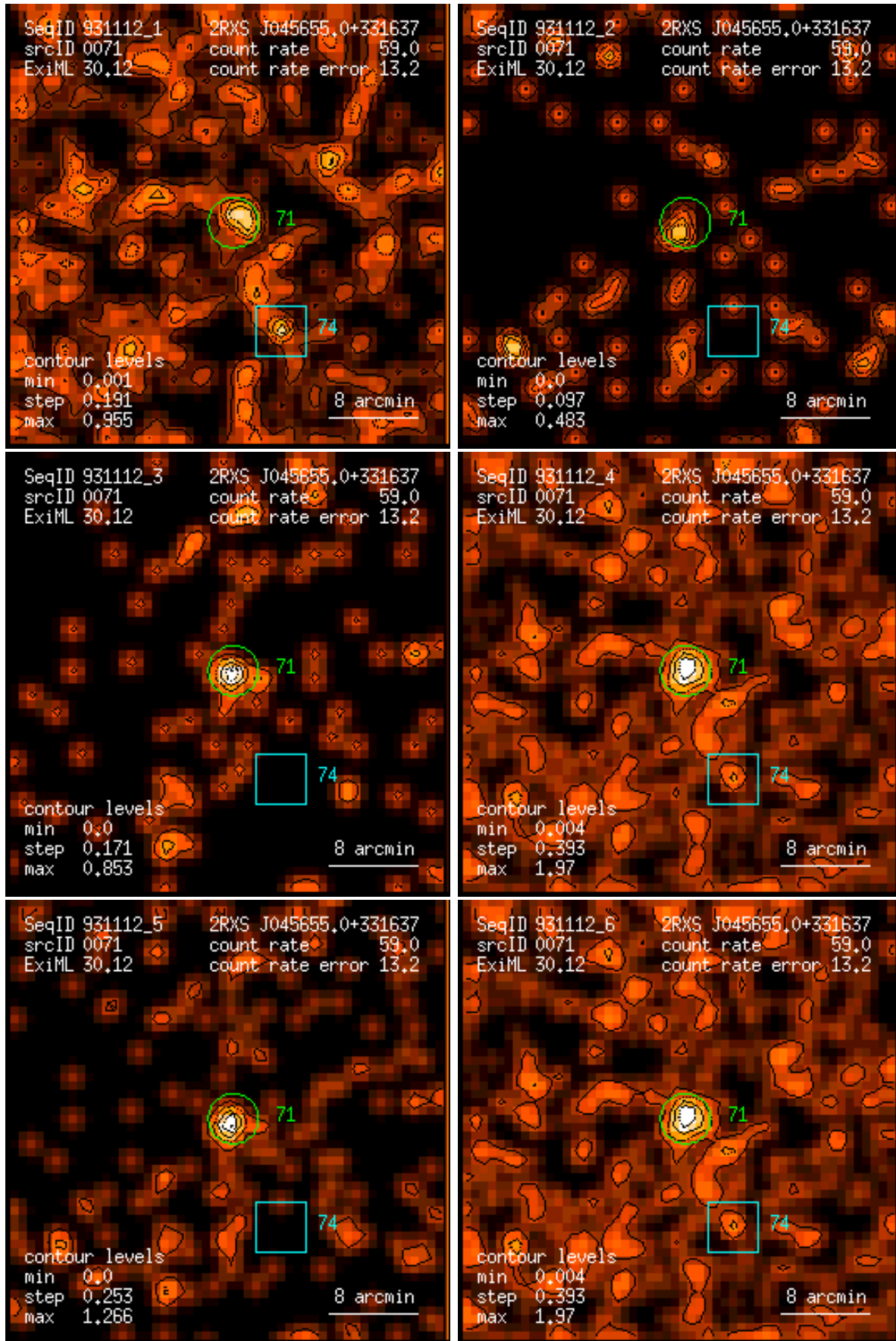
Figure 71: RASS 931112: detection 0071: band rate images, Gaussian filter: (1) PSPC channels 11 – 41, (2) 52 – 90, (3) 91 – 201, (4) 11 – 235, (5) 52 – 201, (6) 11 – 201. Broad band rates in counts/ks. Band rate contour levels in counts/ks/arcmin 2 .
