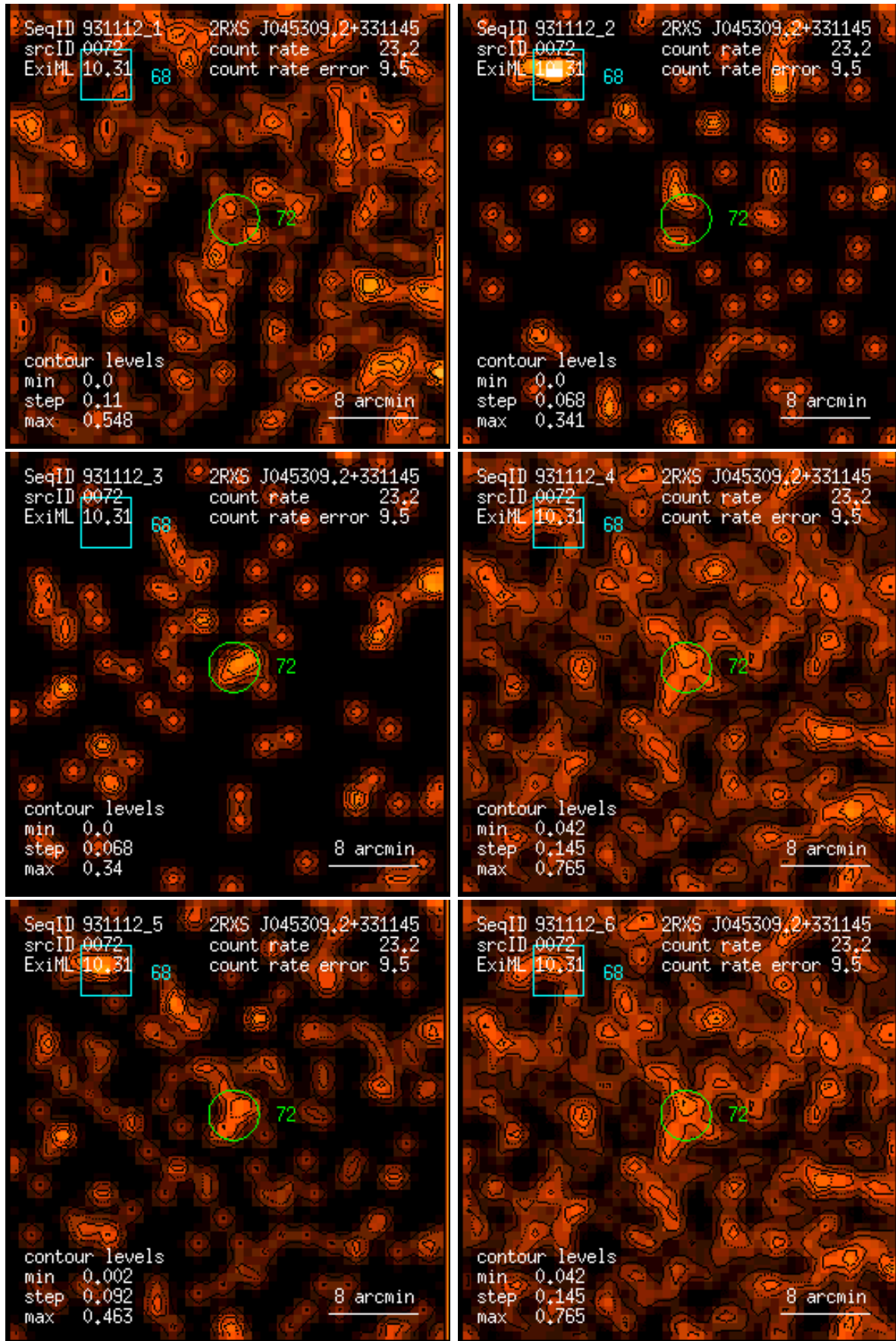
Figure 72: RASS 931112: detection 0072: band rate images, Gaussian filter: (1) PSPC channels 11 – 41, (2) 52 – 90, (3) 91 – 201, (4) 11 – 235, (5) 52 – 201, (6) 11 – 201. Broad band rates in counts/ks. Band rate contour levels in counts/ks/arcmin 2 .
