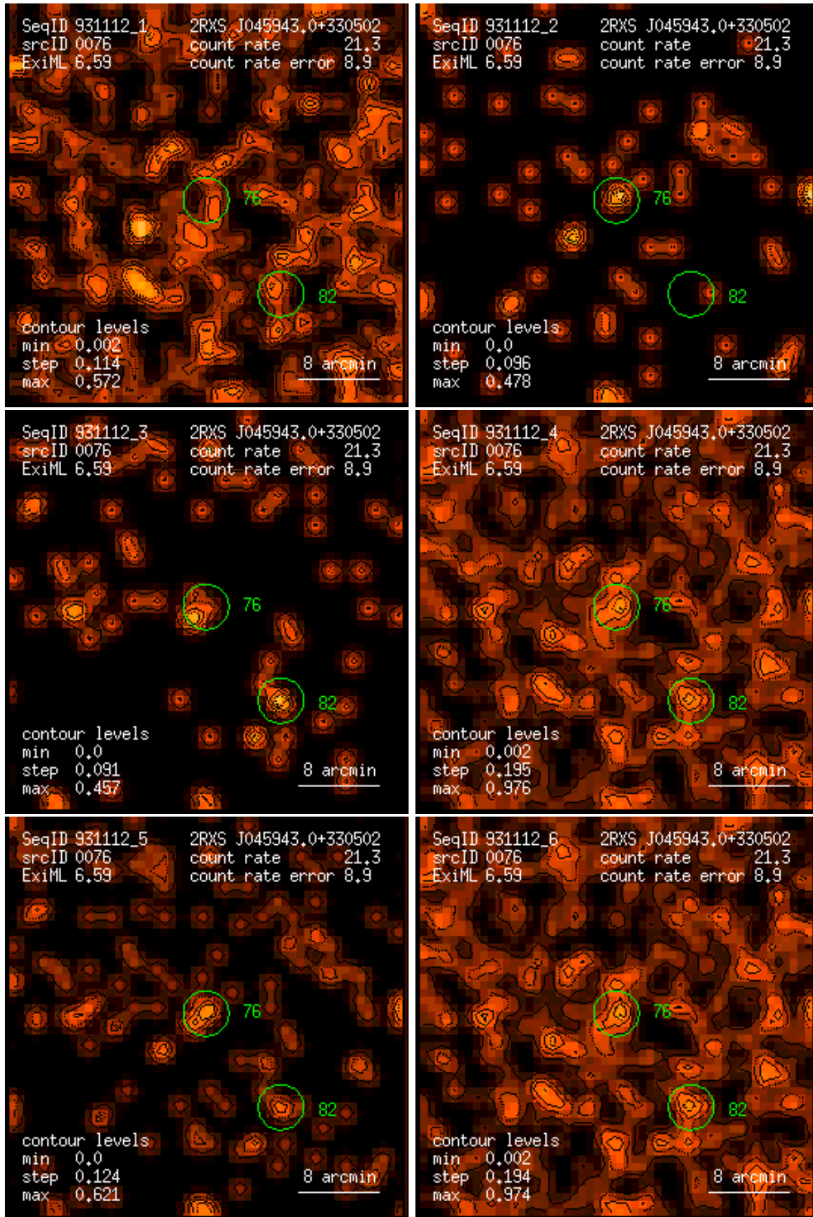
Figure 76: RASS 931112: detection 0076: band rate images, Gaussian filter: (1) PSPC channels 11 – 41, (2) 52 – 90, (3) 91 – 201, (4) 11 – 235, (5) 52 – 201, (6) 11 – 201. Broad band rates in counts/ks. Band rate contour levels in counts/ks/arcmin 2 .
