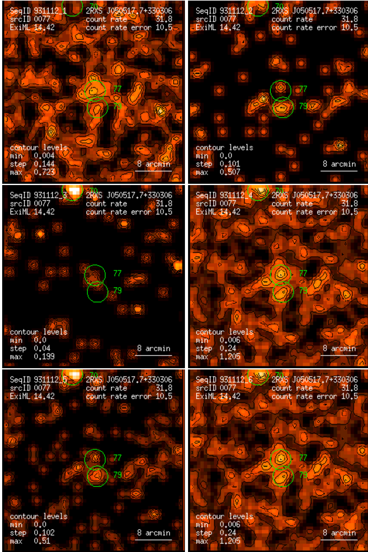
Figure 77: RASS 931112: detection 0077: band rate images, Gaussian filter: (1) PSPC channels 11 – 41, (2) 52 – 90, (3) 91 – 201, (4) 11 – 235, (5) 52 – 201, (6) 11 – 201. Broad band rates in counts/ks. Band rate contour levels in counts/ks/arcmin 2 .
