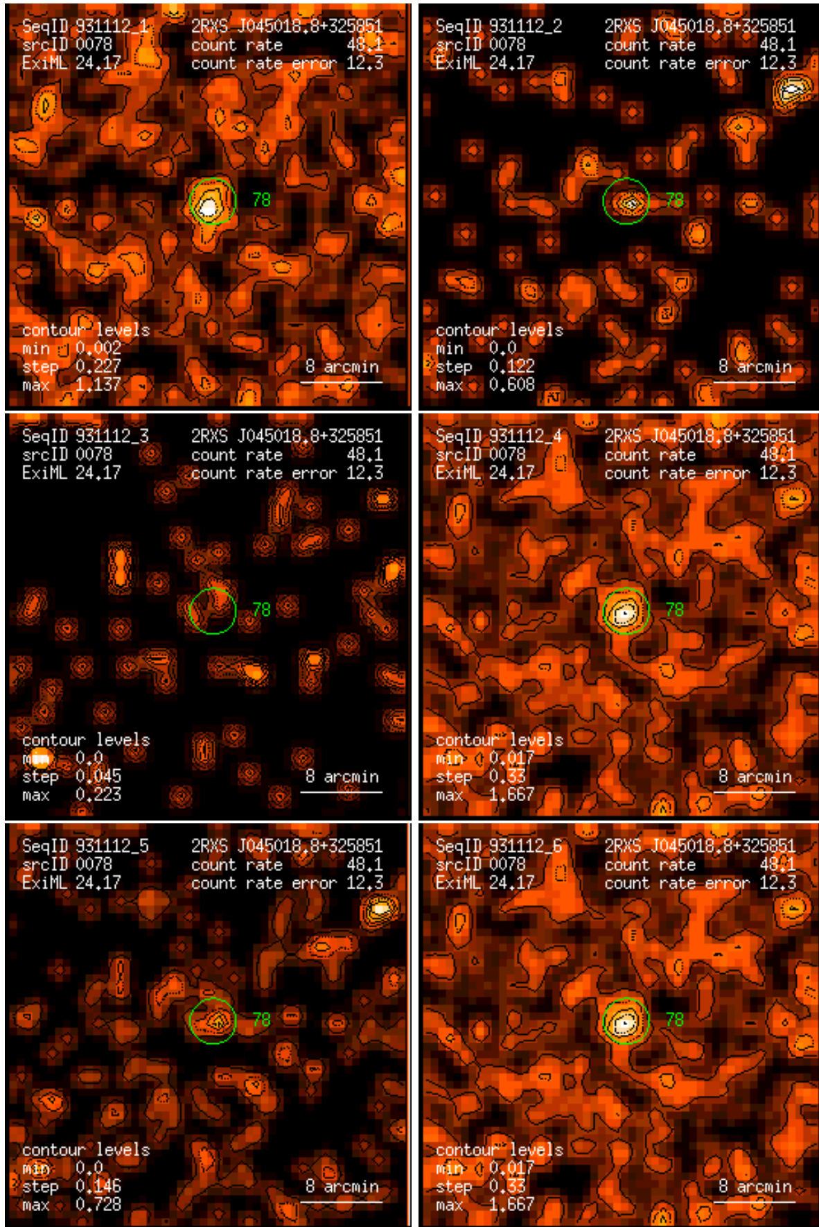
Figure 78: RASS 931112: detection 0078: band rate images, Gaussian filter: (1) PSPC channels 11 – 41, (2) 52 – 90, (3) 91 – 201, (4) 11 – 235, (5) 52 – 201, (6) 11 – 201. Broad band rates in counts/ks. Band rate contour levels in counts/ks/arcmin 2 .
