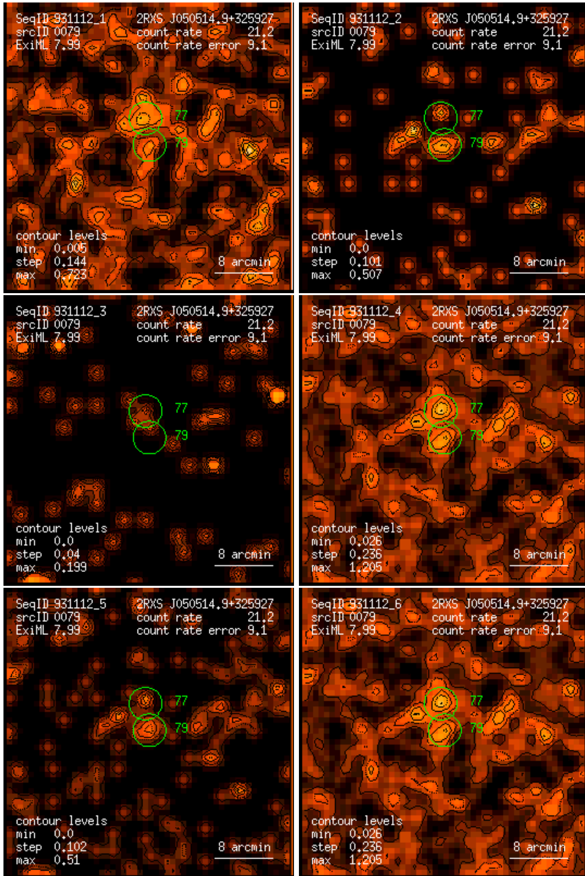
Figure 79: RASS 931112: detection 0079: band rate images, Gaussian filter: (1) PSPC channels 11 – 41, (2) 52 – 90, (3) 91 – 201, (4) 11 – 235, (5) 52 – 201, (6) 11 – 201. Broad band rates in counts/ks. Band rate contour levels in counts/ks/arcmin 2 .
