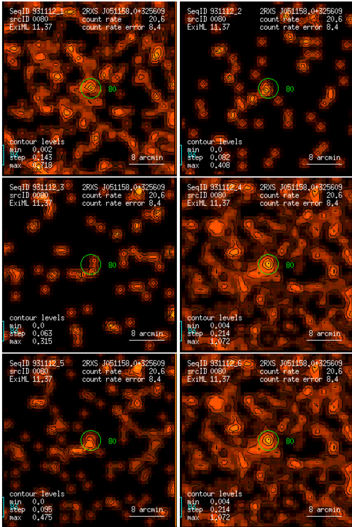
Figure 80: RASS 931112: detection 0080: band rate images, Gaussian filter: (1) PSPC channels 11 – 41, (2) 52 – 90, (3) 91 – 201, (4) 11 – 235, (5) 52 – 201, (6) 11 – 201. Broad band rates in counts/ks. Band rate contour levels in counts/ks/arcmin 2 .
