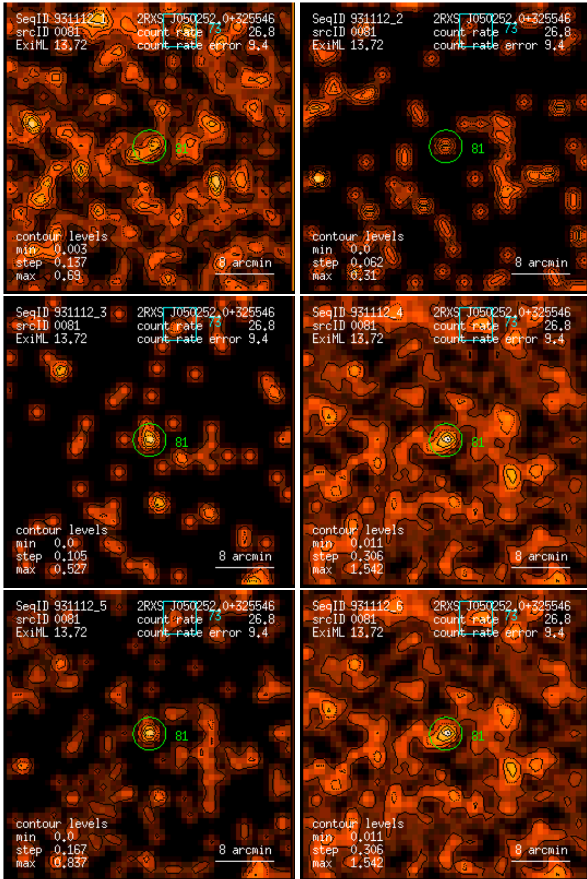
Figure 81: RASS 931112: detection 0081: band rate images, Gaussian filter: (1) PSPC channels 11 – 41, (2) 52 – 90, (3) 91 – 201, (4) 11 – 235, (5) 52 – 201, (6) 11 – 201. Broad band rates in counts/ks. Band rate contour levels in counts/ks/arcmin 2 .
