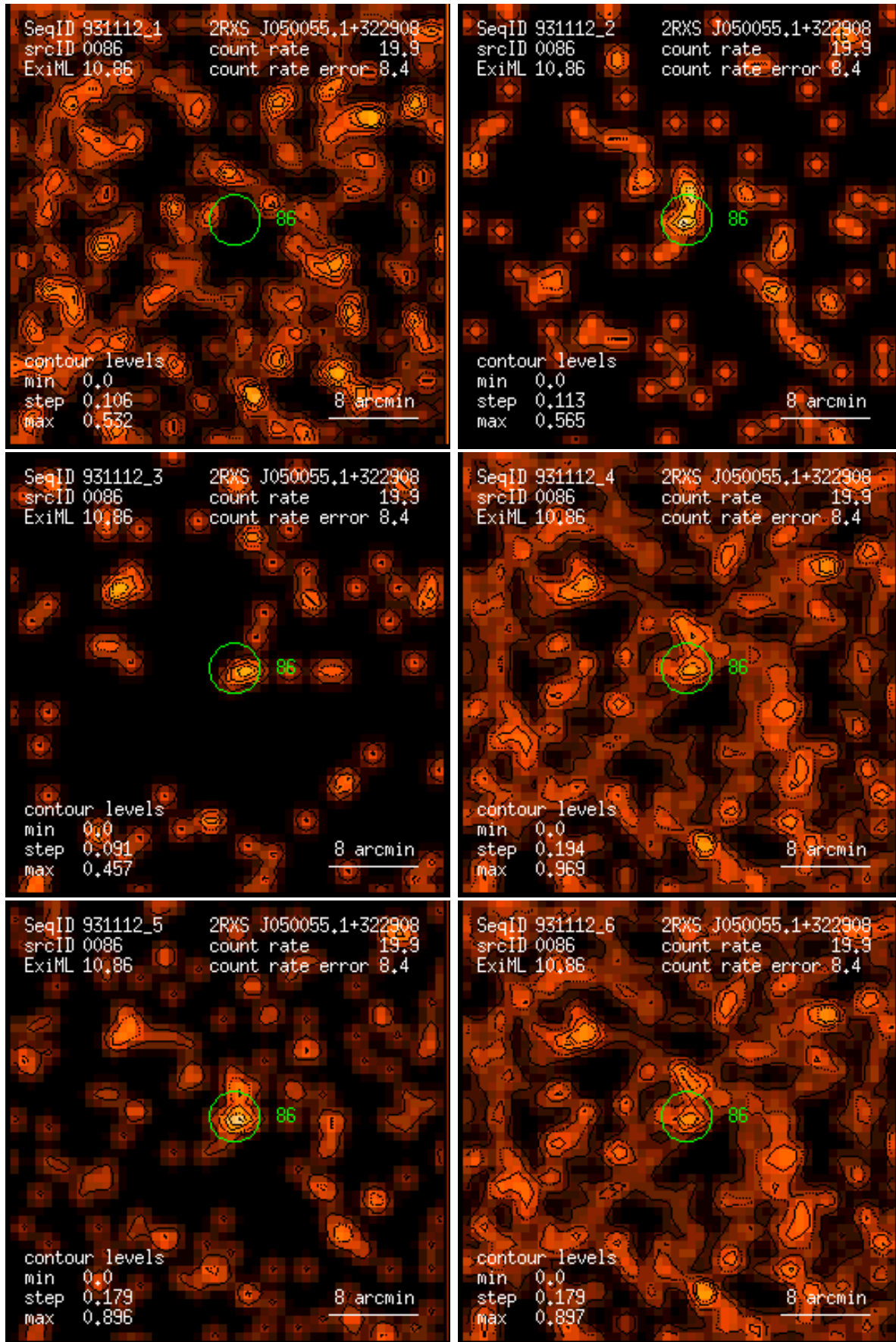
Figure 86: RASS 931112: detection 0086: band rate images, Gaussian filter: (1) PSPC channels 11 – 41, (2) 52 – 90, (3) 91 – 201, (4) 11 – 235, (5) 52 – 201, (6) 11 – 201. Broad band rates in counts/ks. Band rate contour levels in counts/ks/arcmin 2 .
