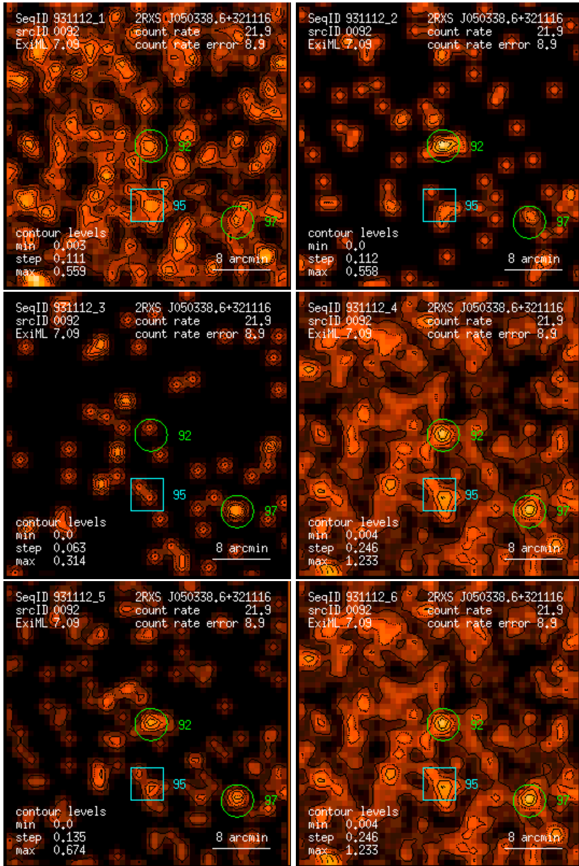
Figure 92: RASS 931112: detection 0092: band rate images, Gaussian filter: (1) PSPC channels 11 – 41, (2) 52 – 90, (3) 91 – 201, (4) 11 – 235, (5) 52 – 201, (6) 11 – 201. Broad band rates in counts/ks. Band rate contour levels in counts/ks/arcmin 2 .
