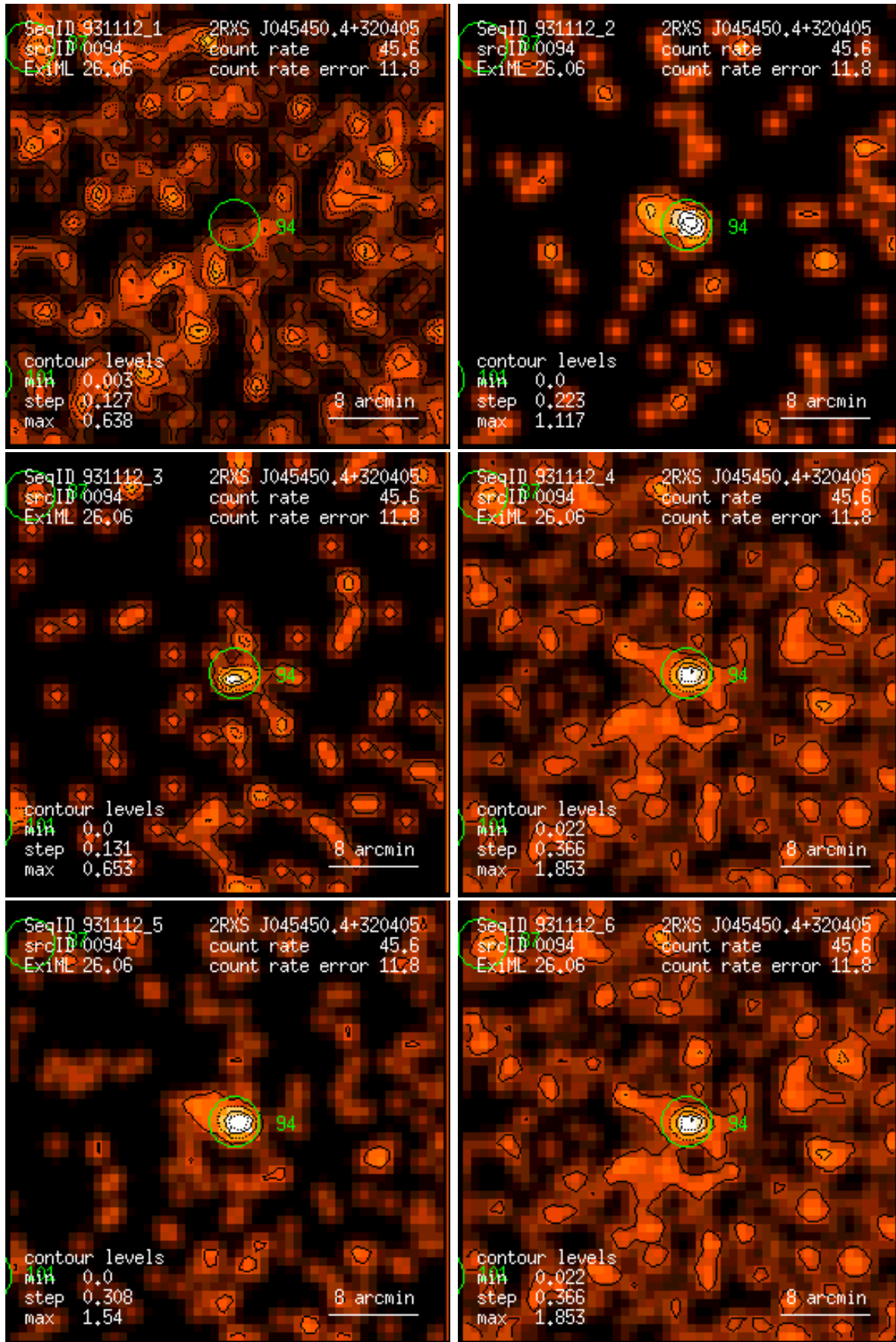
Figure 94: RASS 931112: detection 0094: band rate images, Gaussian filter: (1) PSPC channels 11 – 41, (2) 52 – 90, (3) 91 – 201, (4) 11 – 235, (5) 52 – 201, (6) 11 – 201. Broad band rates in counts/ks. Band rate contour levels in counts/ks/arcmin 2 .
