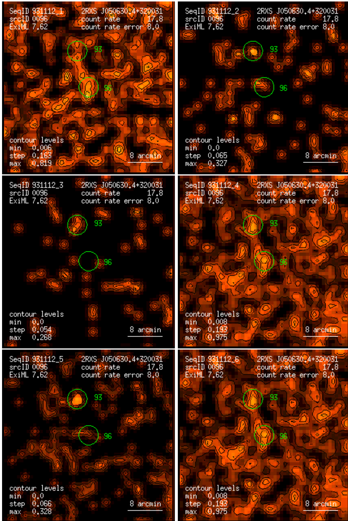
Figure 96: RASS 931112: detection 0096: band rate images, Gaussian filter: (1) PSPC channels 11 – 41, (2) 52 – 90, (3) 91 – 201, (4) 11 – 235, (5) 52 – 201, (6) 11 – 201. Broad band rates in counts/ks. Band rate contour levels in counts/ks/arcmin 2 .
