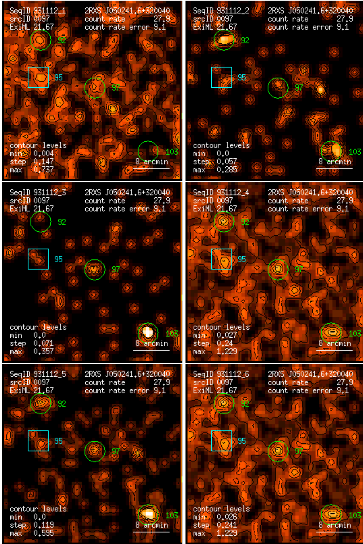
Figure 97: RASS 931112: detection 0097: band rate images, Gaussian filter: (1) PSPC channels 11 – 41, (2) 52 – 90, (3) 91 – 201, (4) 11 – 235, (5) 52 – 201, (6) 11 – 201. Broad band rates in counts/ks. Band rate contour levels in counts/ks/arcmin 2 .
