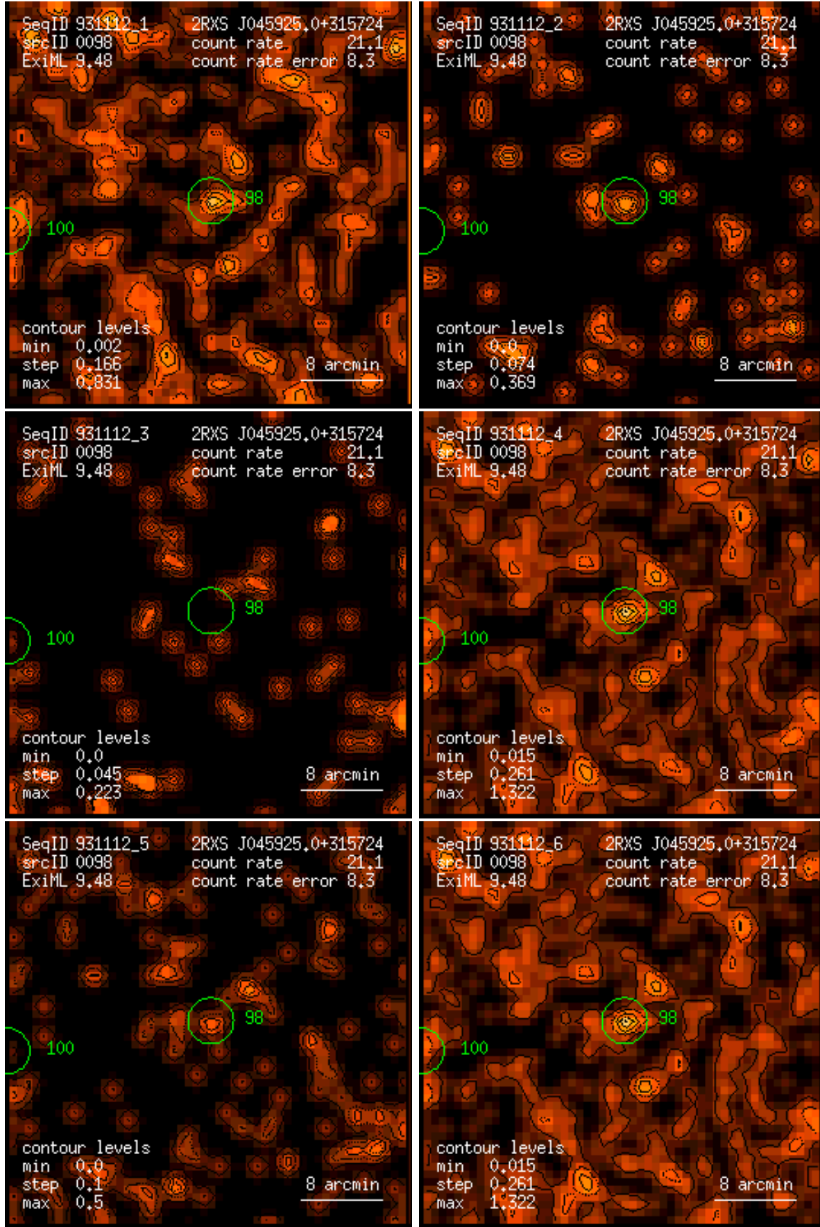
Figure 98: RASS 931112: detection 0098: band rate images, Gaussian filter: (1) PSPC channels 11 – 41, (2) 52 – 90, (3) 91 – 201, (4) 11 – 235, (5) 52 – 201, (6) 11 – 201. Broad band rates in counts/ks. Band rate contour levels in counts/ks/arcmin 2 .
