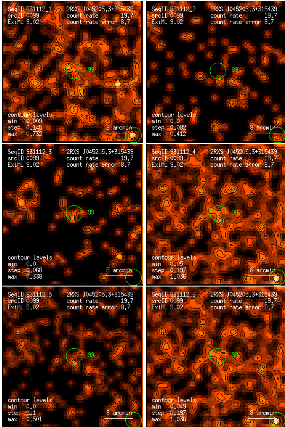
Figure 99: RASS 931112: detection 0099: band rate images, Gaussian filter: (1) PSPC channels 11 – 41, (2) 52 – 90, (3) 91 – 201, (4) 11 – 235, (5) 52 – 201, (6) 11 – 201. Broad band rates in counts/ks. Band rate contour levels in counts/ks/arcmin 2 .
