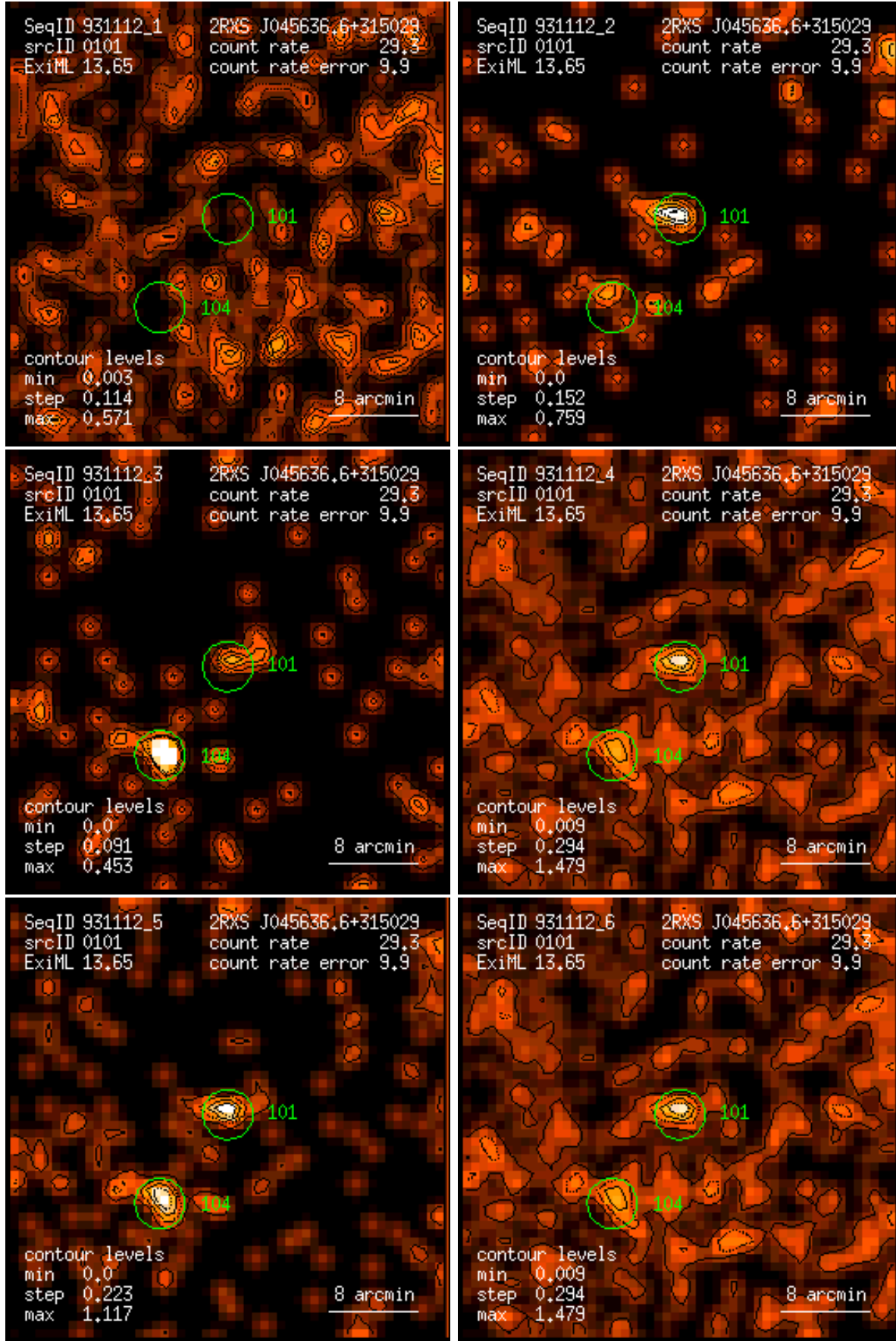
Figure 101: RASS 931112: detection 0101: band rate images, Gaussian filter: (1) PSPC channels 11 – 41, (2) 52 – 90, (3) 91 – 201, (4) 11 – 235, (5) 52 – 201, (6) 11 – 201. Broad band rates in counts/ks. Band rate contour levels in counts/ks/arcmin 2 .
