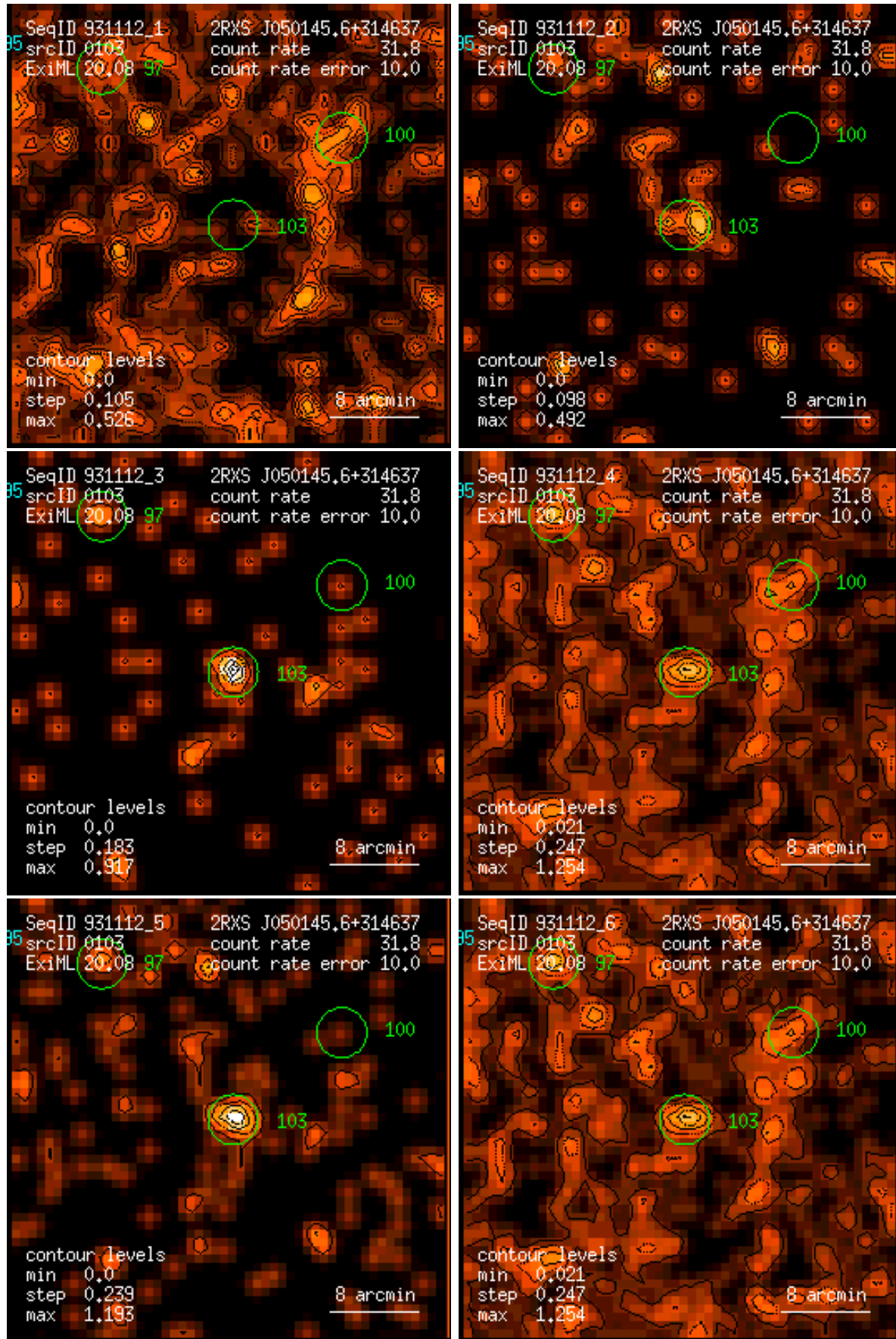
Figure 103: RASS 931112: detection 0103: band rate images, Gaussian filter: (1) PSPC channels 11 – 41, (2) 52 – 90, (3) 91 – 201, (4) 11 – 235, (5) 52 – 201, (6) 11 – 201. Broad band rates in counts/ks. Band rate contour levels in counts/ks/arcmin 2 .
