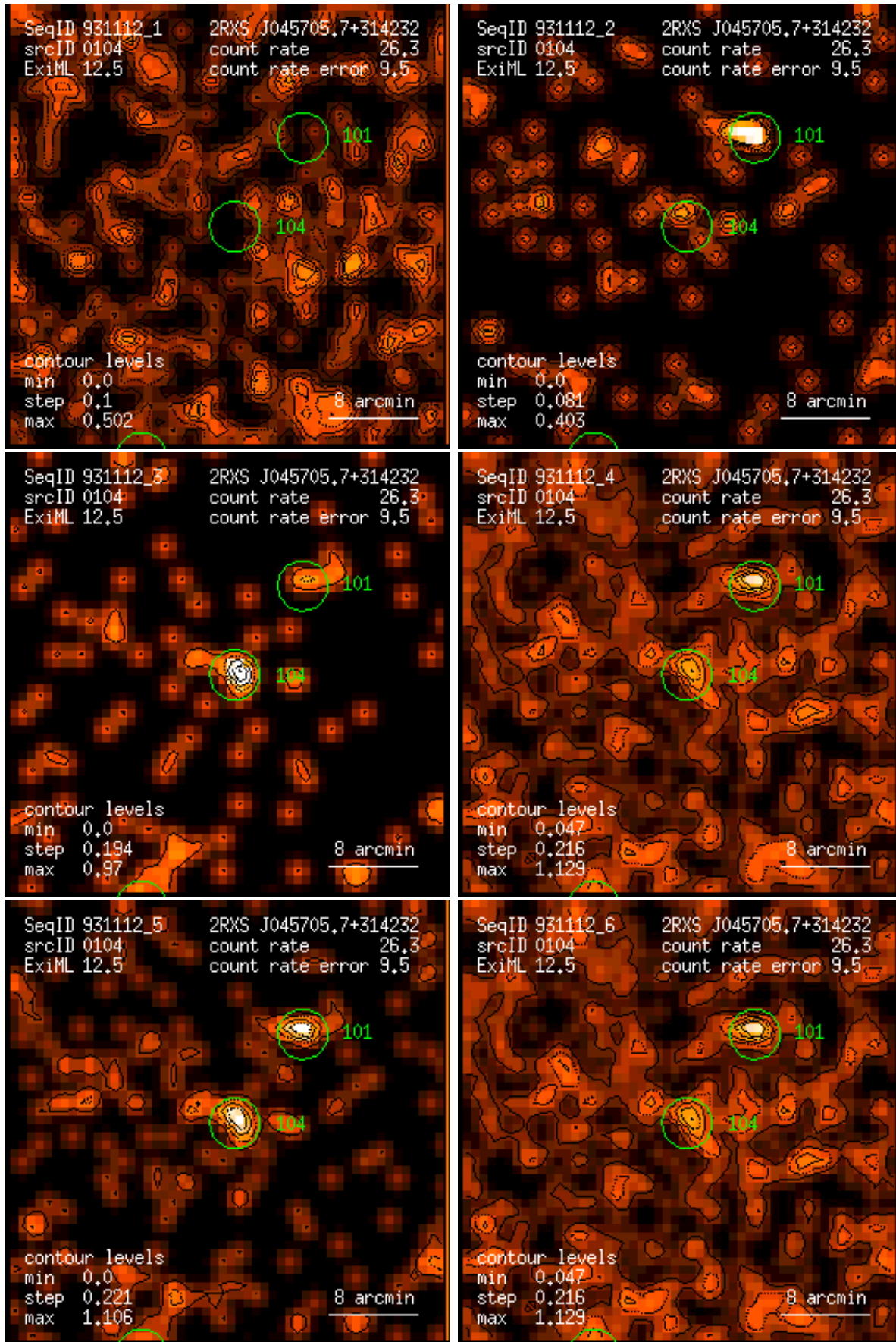
Figure 104: RASS 931112: detection 0104: band rate images, Gaussian filter: (1) PSPC channels 11 – 41, (2) 52 – 90, (3) 91 – 201, (4) 11 – 235, (5) 52 – 201, (6) 11 – 201. Broad band rates in counts/ks. Band rate contour levels in counts/ks/arcmin 2 .
