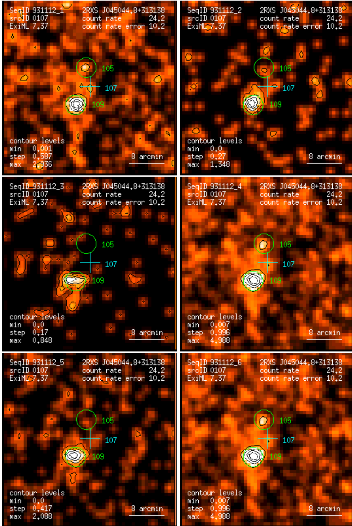
Figure 107: RASS 931112: detection 0107: band rate images, Gaussian filter: (1) PSPC channels 11 – 41, (2) 52 – 90, (3) 91 – 201, (4) 11 – 235, (5) 52 – 201, (6) 11 – 201. Broad band rates in counts/ks. Band rate contour levels in counts/ks/arcmin 2 .
