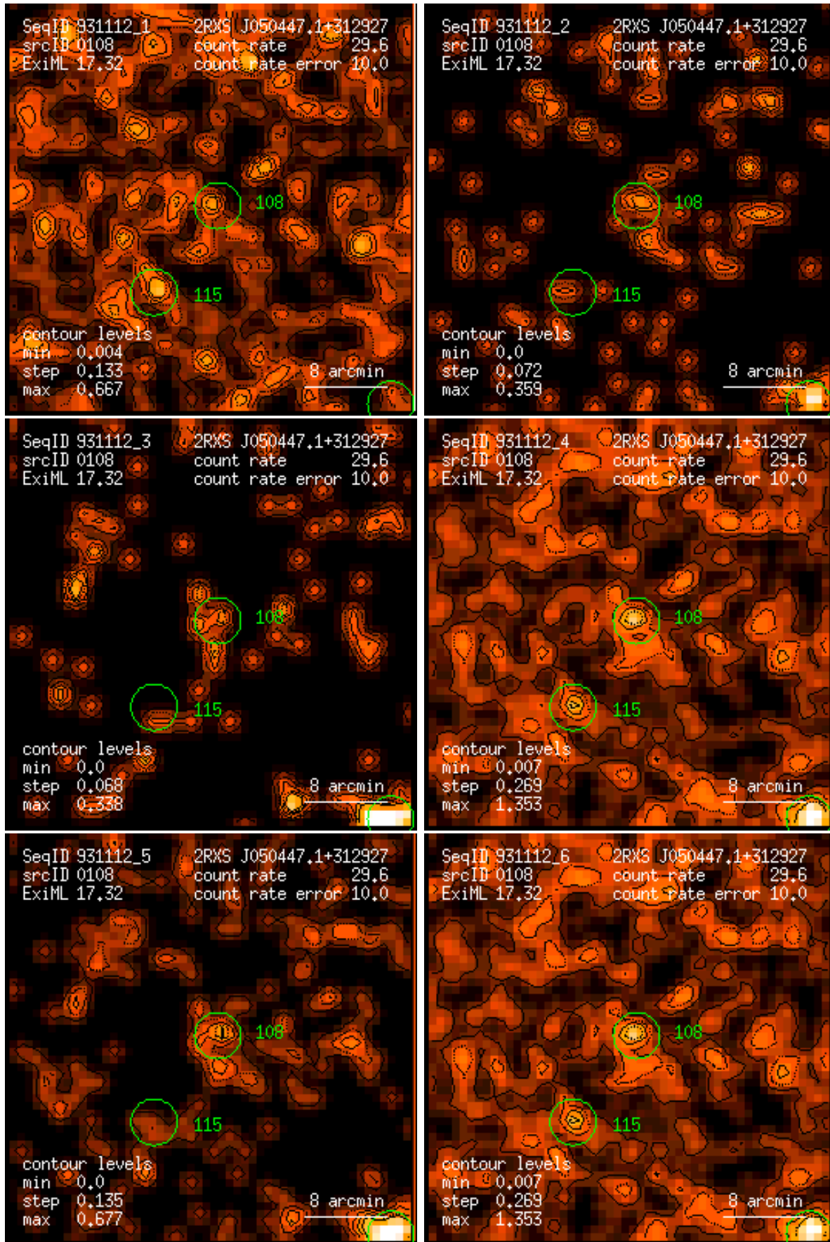
Figure 108: RASS 931112: detection 0108: band rate images, Gaussian filter: (1) PSPC channels 11 – 41, (2) 52 – 90, (3) 91 – 201, (4) 11 – 235, (5) 52 – 201, (6) 11 – 201. Broad band rates in counts/ks. Band rate contour levels in counts/ks/arcmin 2 .
