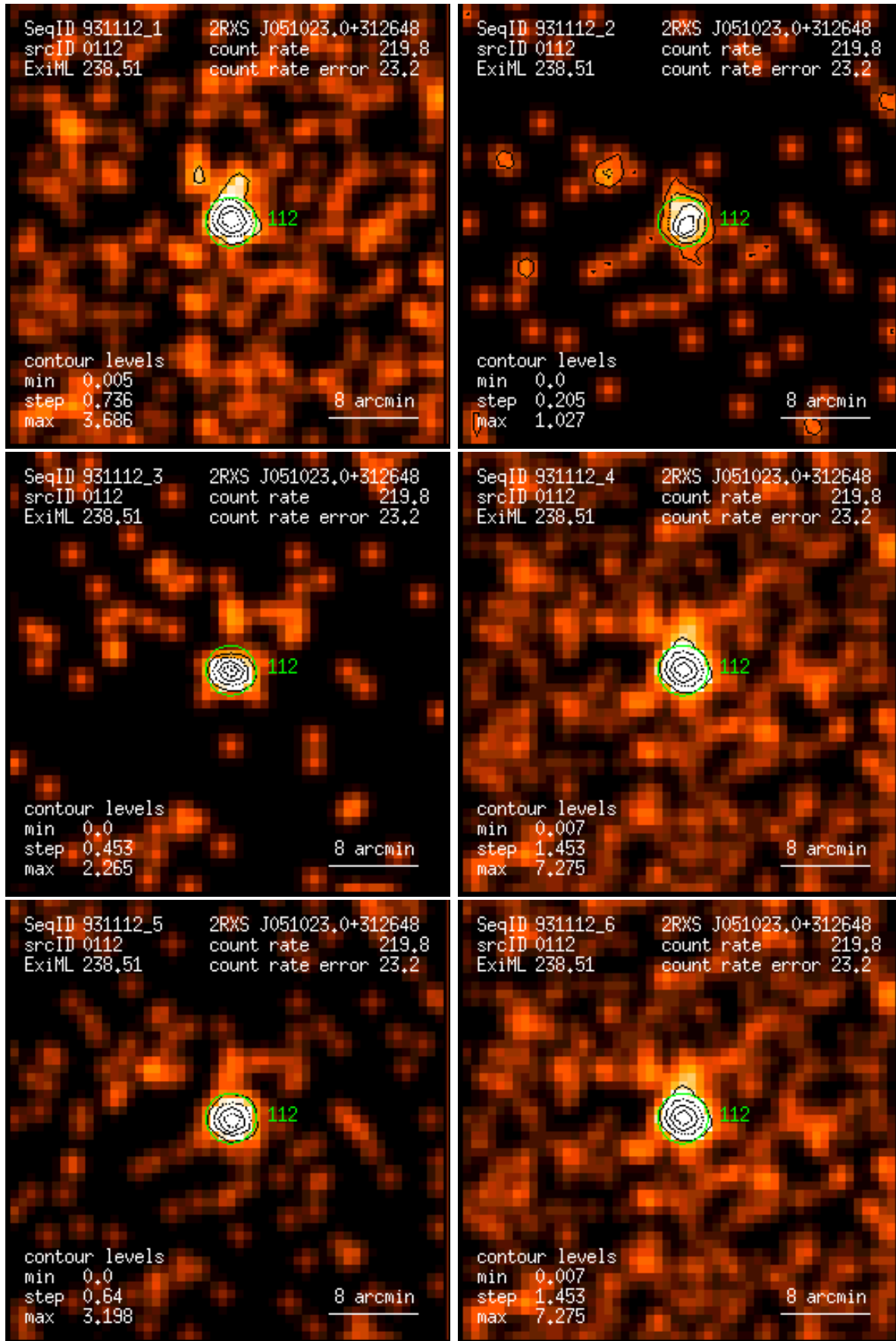
Figure 112: RASS 931112: detection 0112: band rate images, Gaussian filter: (1) PSPC channels 11 – 41, (2) 52 – 90, (3) 91 – 201, (4) 11 – 235, (5) 52 – 201, (6) 11 – 201. Broad band rates in counts/ks. Band rate contour levels in counts/ks/arcmin 2 .
