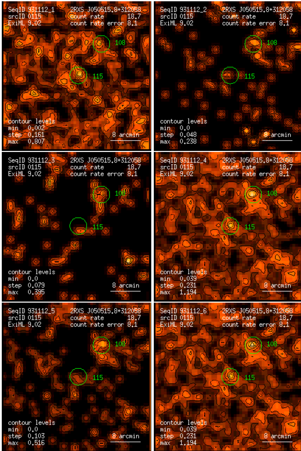
Figure 115: RASS 931112: detection 0115: band rate images, Gaussian filter: (1) PSPC channels 11 – 41, (2) 52 – 90, (3) 91 – 201, (4) 11 – 235, (5) 52 – 201, (6) 11 – 201. Broad band rates in counts/ks. Band rate contour levels in counts/ks/arcmin 2 .
