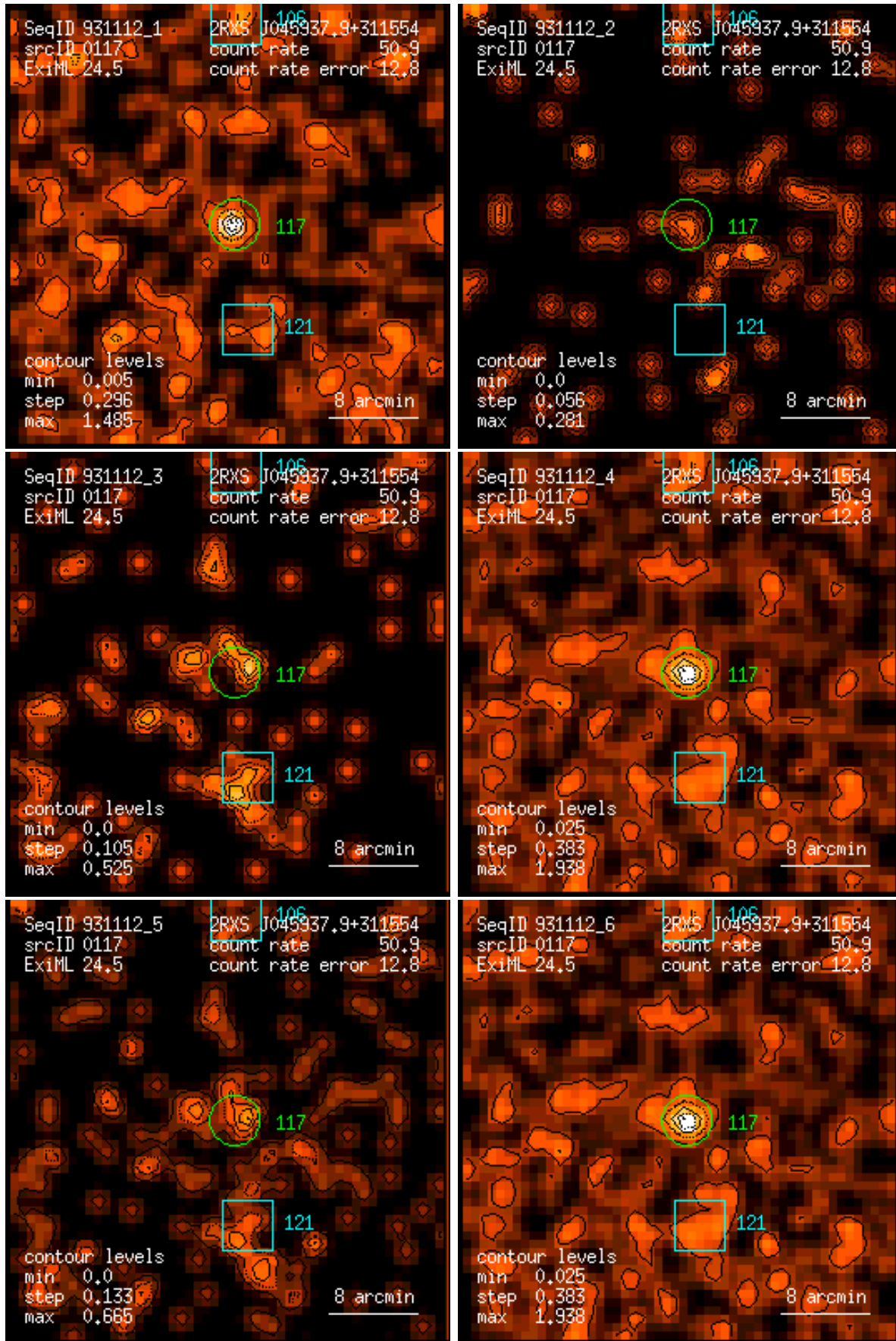
Figure 117: RASS 931112: detection 0117: band rate images, Gaussian filter: (1) PSPC channels 11 – 41, (2) 52 – 90, (3) 91 – 201, (4) 11 – 235, (5) 52 – 201, (6) 11 – 201. Broad band rates in counts/ks. Band rate contour levels in counts/ks/arcmin 2 .
