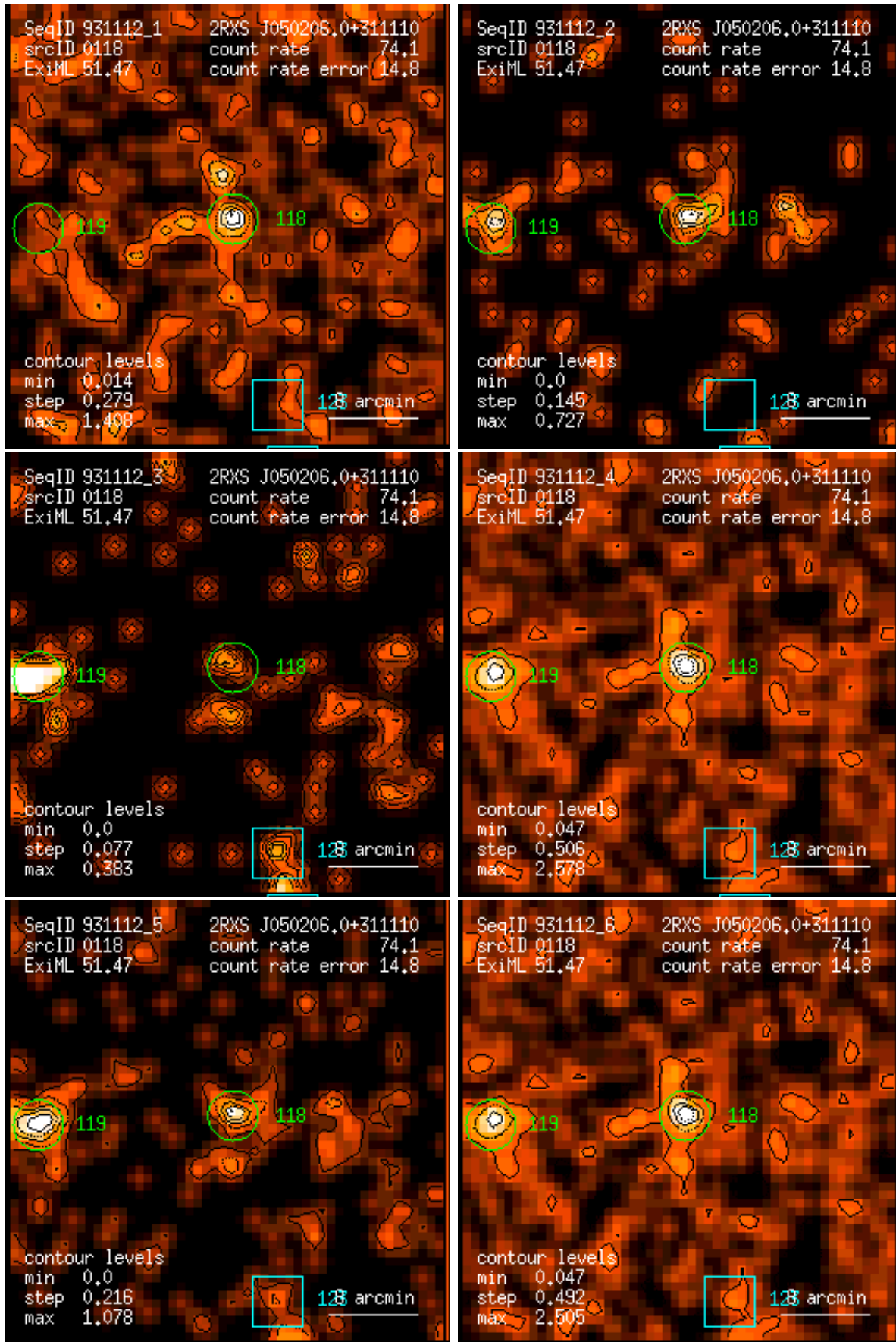
Figure 118: RASS 931112: detection 0118: band rate images, Gaussian filter: (1) PSPC channels 11 – 41, (2) 52 – 90, (3) 91 – 201, (4) 11 – 235, (5) 52 – 201, (6) 11 – 201. Broad band rates in counts/ks. Band rate contour levels in counts/ks/arcmin 2 .
