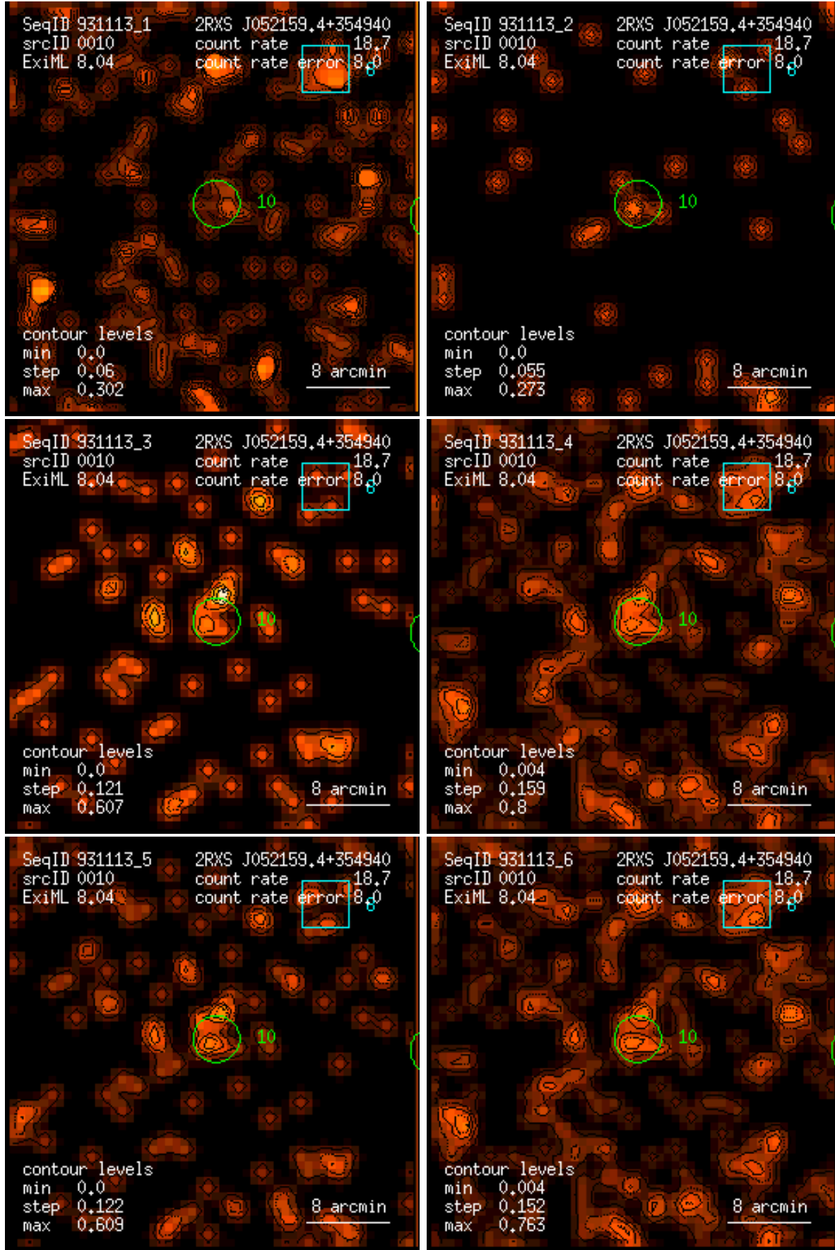
Figure 10: RASS 931113: detection 0010: band rate images, Gaussian filter: (1) PSPC channels 11 – 41, (2) 52 – 90, (3) 91 – 201, (4) 11 – 235, (5) 52 – 201, (6) 11 – 201. Broad band rates in counts/ks. Band rate contour levels in counts/ks/arcmin 2 .
