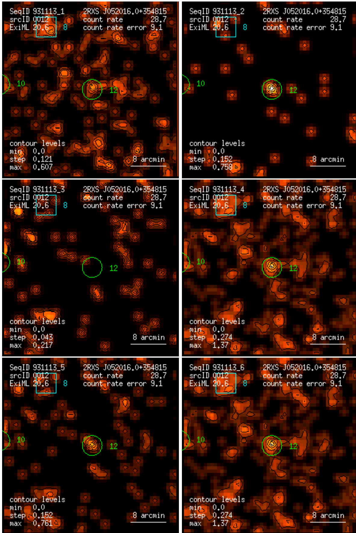
Figure 12: RASS 931113: detection 0012: band rate images, Gaussian filter: (1) PSPC channels 11 – 41, (2) 52 – 90, (3) 91 – 201, (4) 11 – 235, (5) 52 – 201, (6) 11 – 201. Broad band rates in counts/ks. Band rate contour levels in counts/ks/arcmin 2 .
