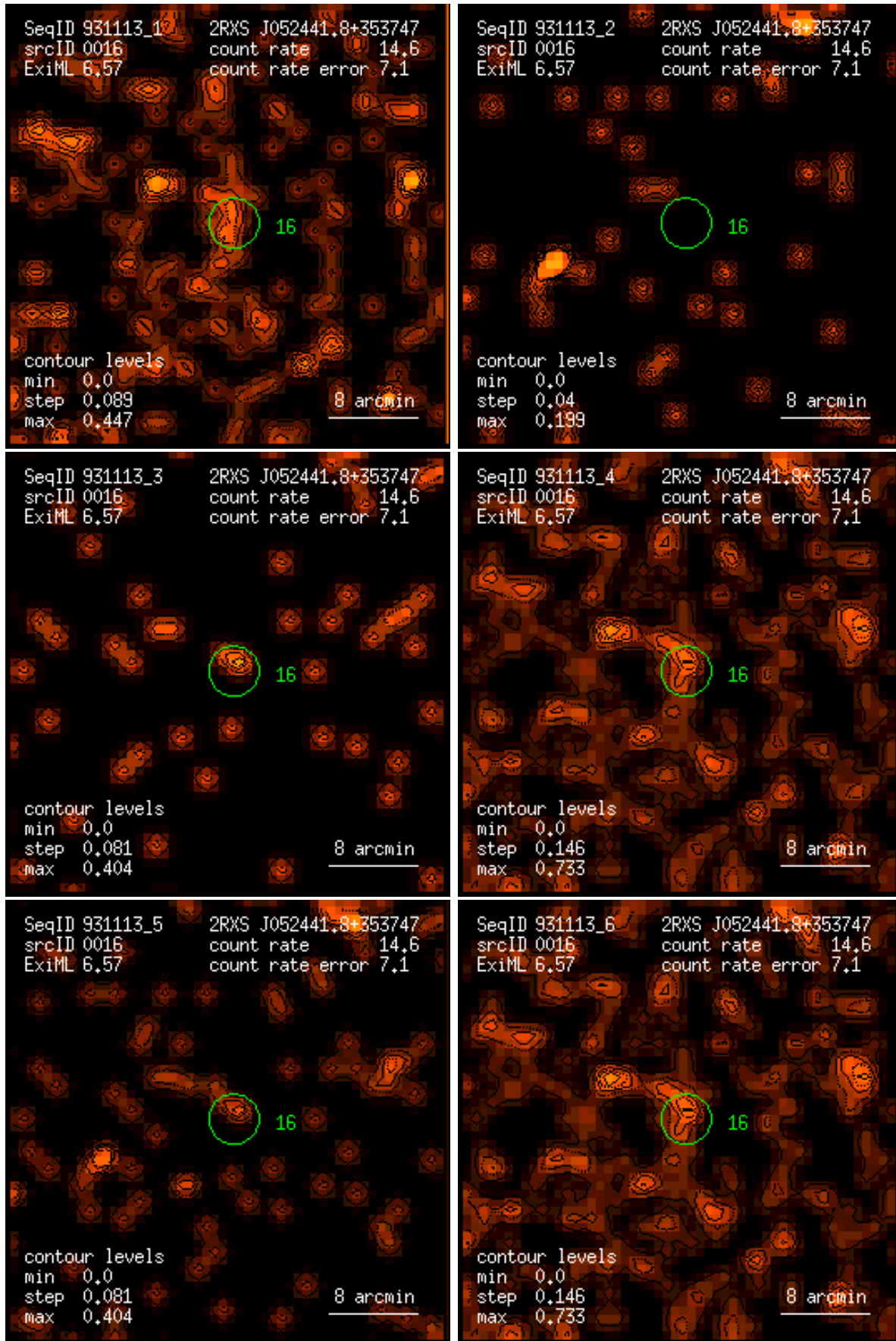
Figure 16: RASS 931113: detection 0016: band rate images, Gaussian filter: (1) PSPC channels 11 – 41, (2) 52 – 90, (3) 91 – 201, (4) 11 – 235, (5) 52 – 201, (6) 11 – 201. Broad band rates in counts/ks. Band rate contour levels in counts/ks/arcmin 2 .
