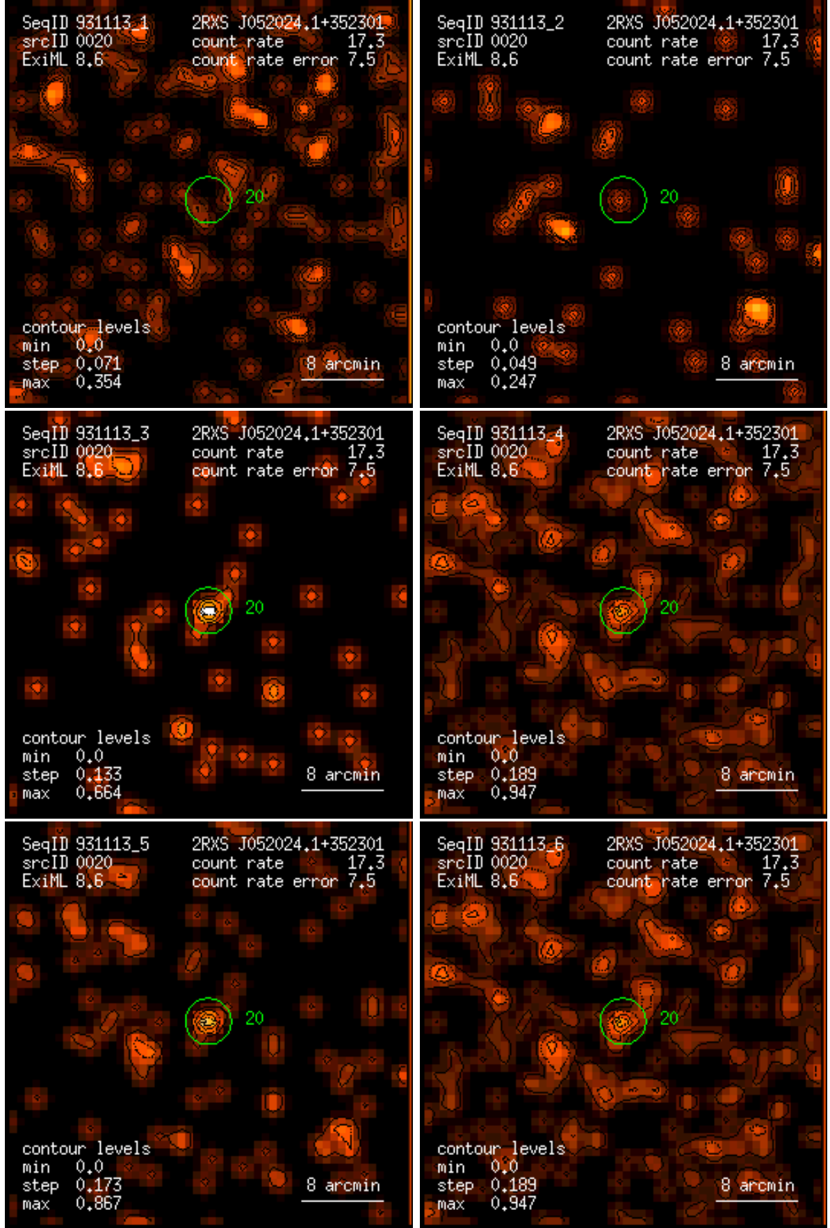
Figure 20: RASS 931113: detection 0020: band rate images, Gaussian filter: (1) PSPC channels 11 – 41, (2) 52 – 90, (3) 91 – 201, (4) 11 – 235, (5) 52 – 201, (6) 11 – 201. Broad band rates in counts/ks. Band rate contour levels in counts/ks/arcmin 2 .
