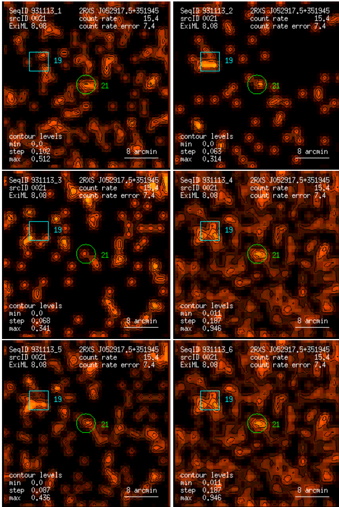
Figure 21: RASS 931113: detection 0021: band rate images, Gaussian filter: (1) PSPC channels 11 – 41, (2) 52 – 90, (3) 91 – 201, (4) 11 – 235, (5) 52 – 201, (6) 11 – 201. Broad band rates in counts/ks. Band rate contour levels in counts/ks/arcmin 2 .
