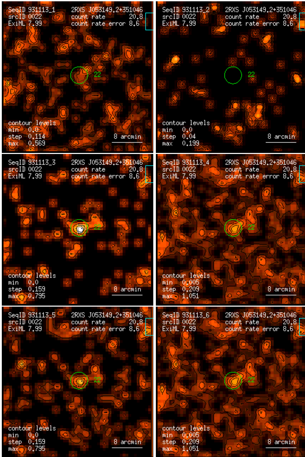
Figure 22: RASS 931113: detection 0022: band rate images, Gaussian filter: (1) PSPC channels 11 – 41, (2) 52 – 90, (3) 91 – 201, (4) 11 – 235, (5) 52 – 201, (6) 11 – 201. Broad band rates in counts/ks. Band rate contour levels in counts/ks/arcmin 2 .
