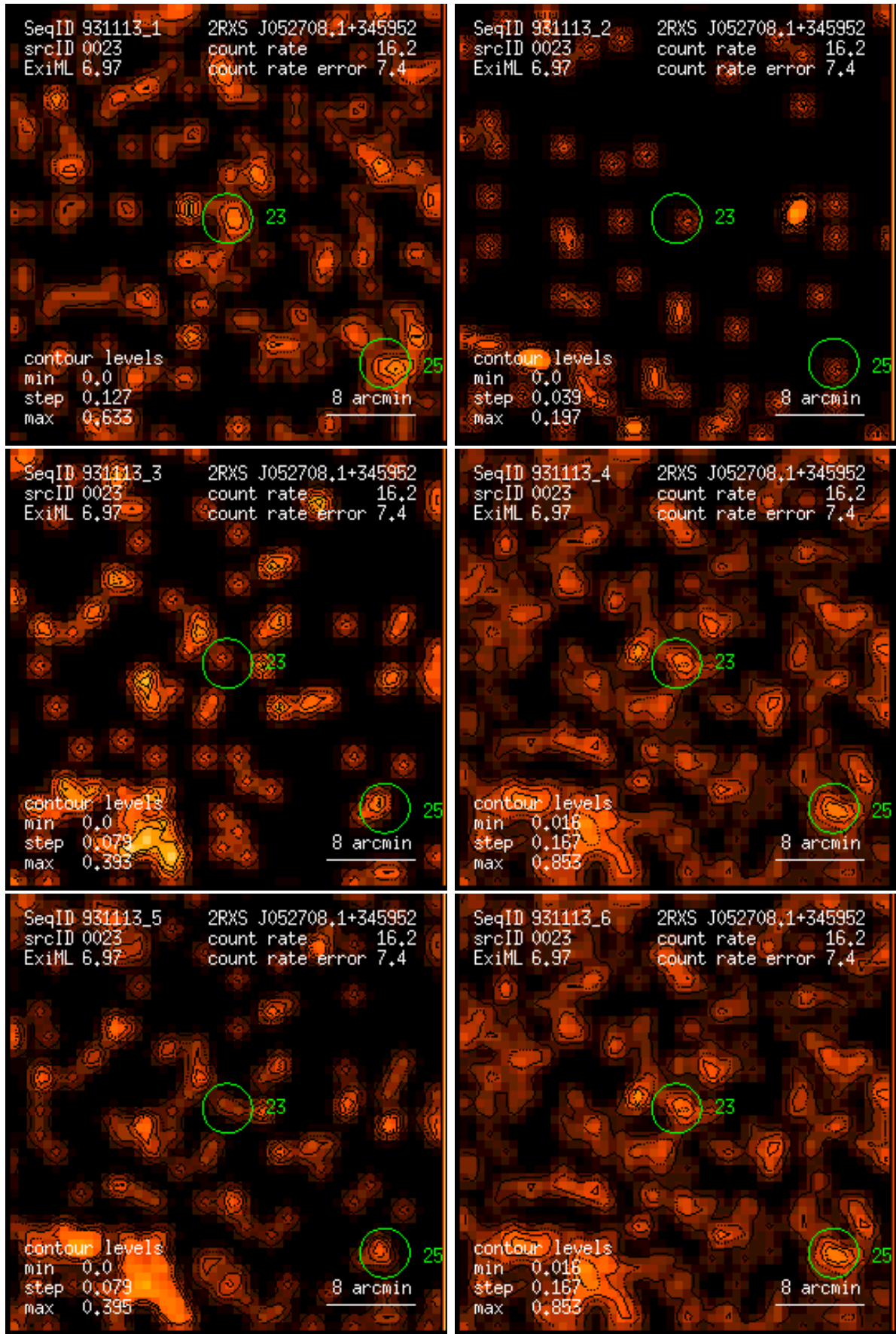
Figure 23: RASS 931113: detection 0023: band rate images, Gaussian filter: (1) PSPC channels 11 – 41, (2) 52 – 90, (3) 91 – 201, (4) 11 – 235, (5) 52 – 201, (6) 11 – 201. Broad band rates in counts/ks. Band rate contour levels in counts/ks/arcmin 2 .
