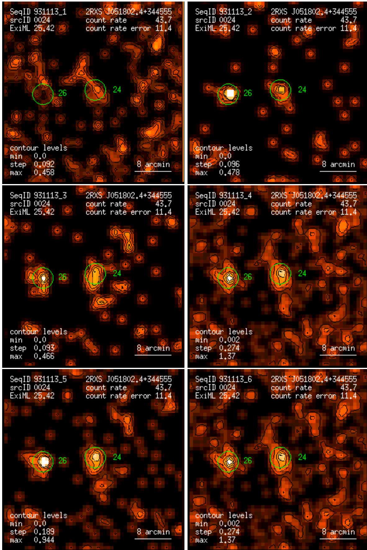
Figure 24: RASS 931113: detection 0024: band rate images, Gaussian filter: (1) PSPC channels 11 – 41, (2) 52 – 90, (3) 91 – 201, (4) 11 – 235, (5) 52 – 201, (6) 11 – 201. Broad band rates in counts/ks. Band rate contour levels in counts/ks/arcmin 2 .
