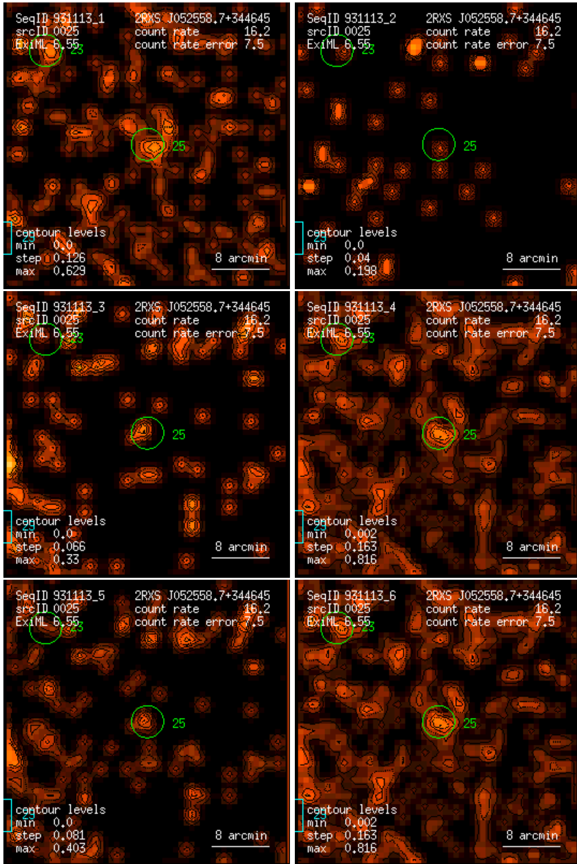
Figure 25: RASS 931113: detection 0025: band rate images, Gaussian filter: (1) PSPC channels 11 – 41, (2) 52 – 90, (3) 91 – 201, (4) 11 – 235, (5) 52 – 201, (6) 11 – 201. Broad band rates in counts/ks. Band rate contour levels in counts/ks/arcmin 2 .
