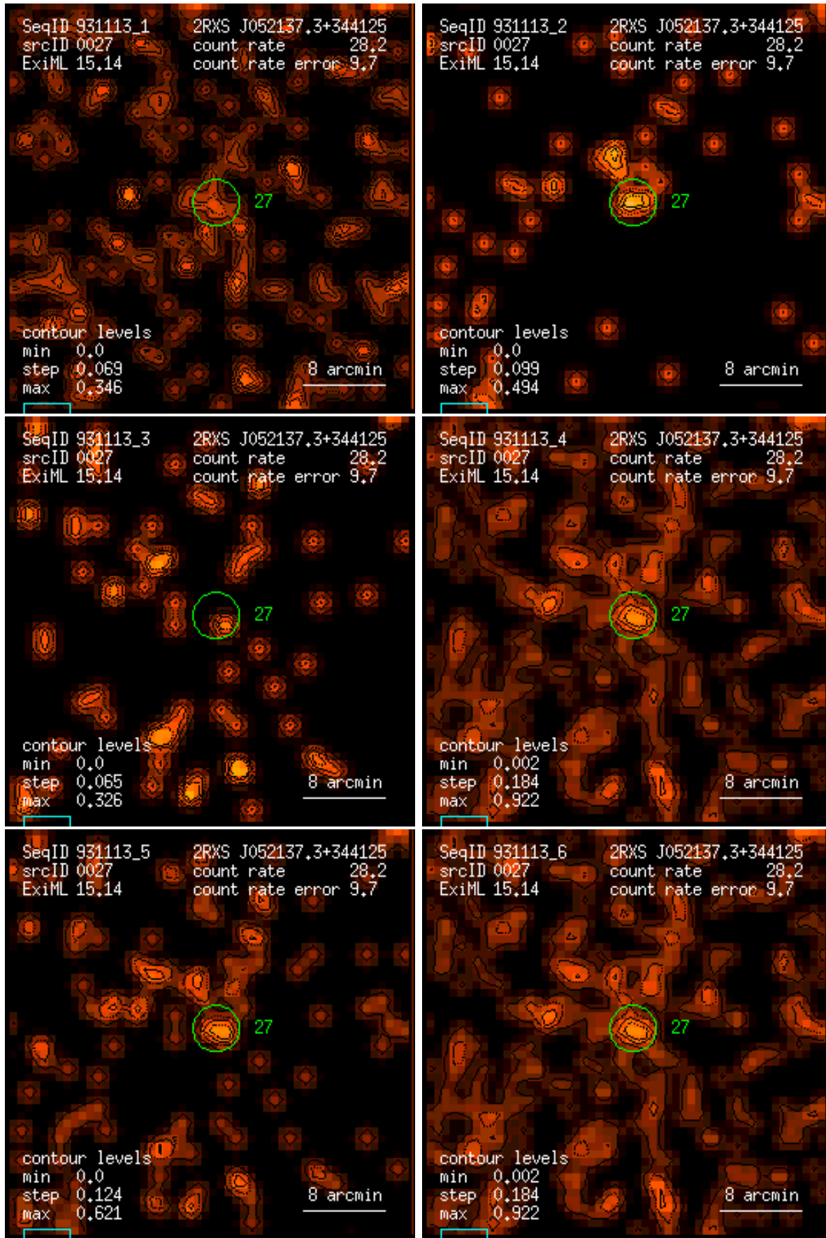
Figure 27: RASS 931113: detection 0027: band rate images, Gaussian filter: (1) PSPC channels 11 – 41, (2) 52 – 90, (3) 91 – 201, (4) 11 – 235, (5) 52 – 201, (6) 11 – 201. Broad band rates in counts/ks. Band rate contour levels in counts/ks/arcmin 2 .
