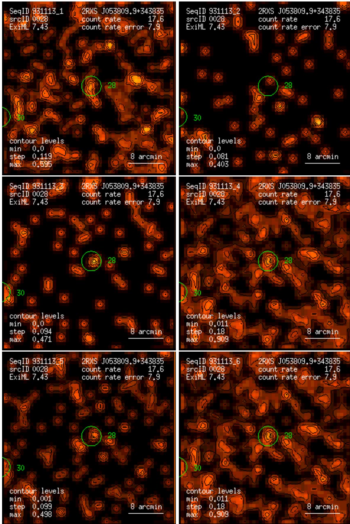
Figure 28: RASS 931113: detection 0028: band rate images, Gaussian filter: (1) PSPC channels 11 – 41, (2) 52 – 90, (3) 91 – 201, (4) 11 – 235, (5) 52 – 201, (6) 11 – 201. Broad band rates in counts/ks. Band rate contour levels in counts/ks/arcmin 2 .
