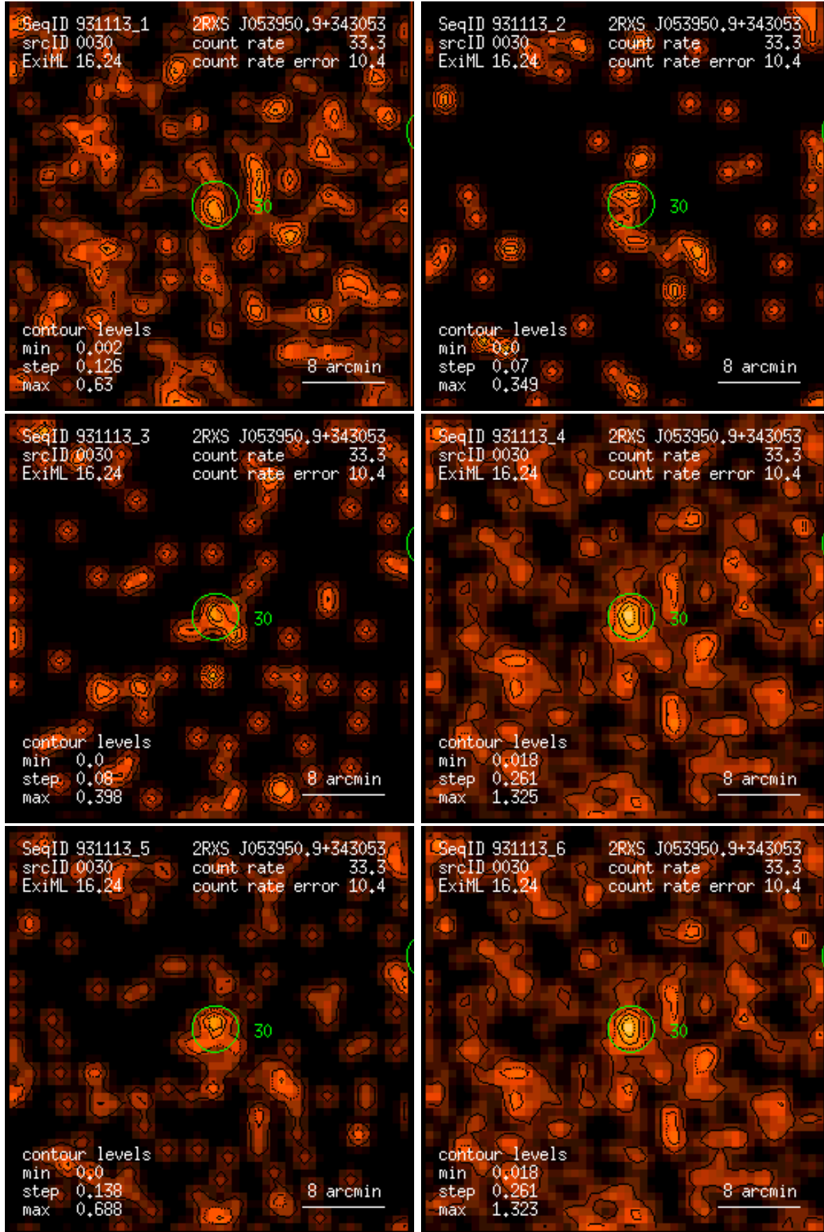
Figure 30: RASS 931113: detection 0030: band rate images, Gaussian filter: (1) PSPC channels 11 – 41, (2) 52 – 90, (3) 91 – 201, (4) 11 – 235, (5) 52 – 201, (6) 11 – 201. Broad band rates in counts/ks. Band rate contour levels in counts/ks/arcmin 2 .
