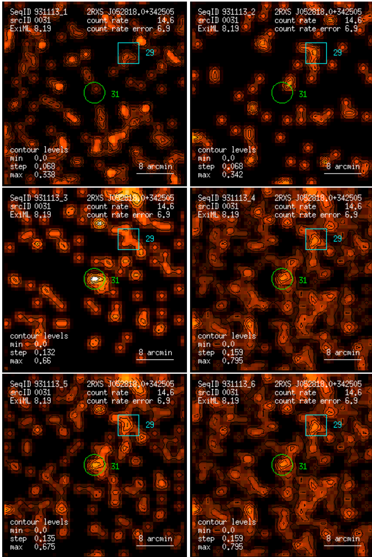
Figure 31: RASS 931113: detection 0031: band rate images, Gaussian filter: (1) PSPC channels 11 – 41, (2) 52 – 90, (3) 91 – 201, (4) 11 – 235, (5) 52 – 201, (6) 11 – 201. Broad band rates in counts/ks. Band rate contour levels in counts/ks/arcmin 2 .
