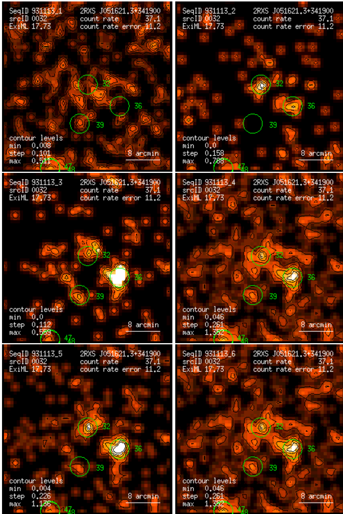
Figure 32: RASS 931113: detection 0032: band rate images, Gaussian filter: (1) PSPC channels 11 – 41, (2) 52 – 90, (3) 91 – 201, (4) 11 – 235, (5) 52 – 201, (6) 11 – 201. Broad band rates in counts/ks. Band rate contour levels in counts/ks/arcmin 2 .
