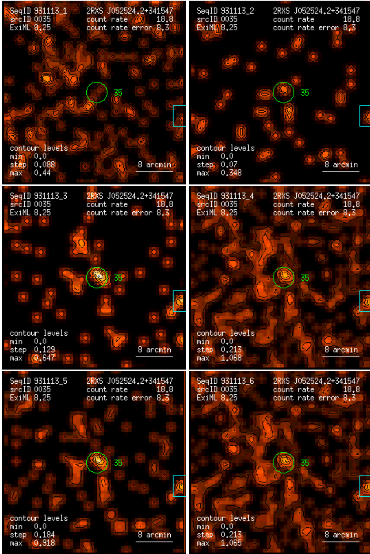
Figure 35: RASS 931113: detection 0035: band rate images, Gaussian filter: (1) PSPC channels 11 – 41, (2) 52 – 90, (3) 91 – 201, (4) 11 – 235, (5) 52 – 201, (6) 11 – 201. Broad band rates in counts/ks. Band rate contour levels in counts/ks/arcmin 2 .
