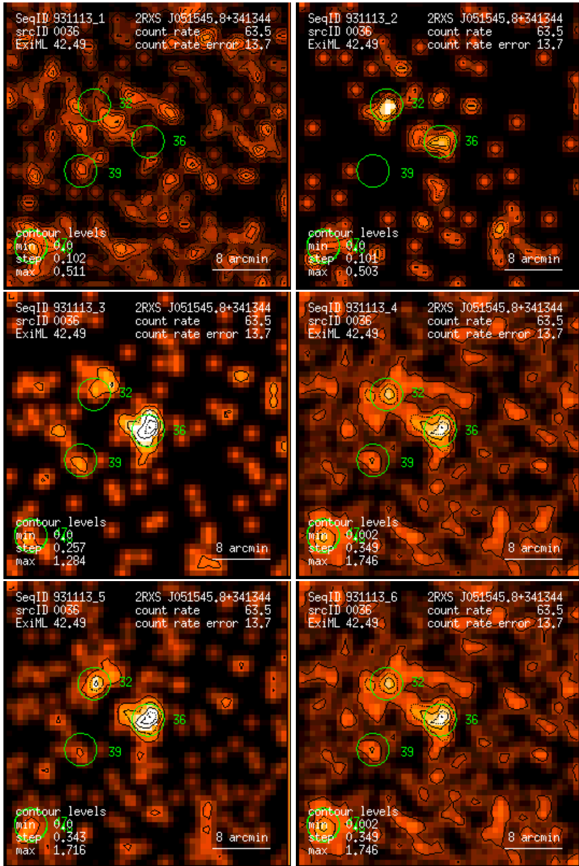
Figure 36: RASS 931113: detection 0036: band rate images, Gaussian filter: (1) PSPC channels 11 – 41, (2) 52 – 90, (3) 91 – 201, (4) 11 – 235, (5) 52 – 201, (6) 11 – 201. Broad band rates in counts/ks. Band rate contour levels in counts/ks/arcmin 2 .
