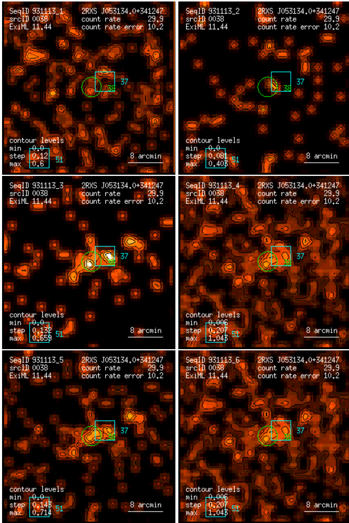
Figure 38: RASS 931113: detection 0038: band rate images, Gaussian filter: (1) PSPC channels 11 – 41, (2) 52 – 90, (3) 91 – 201, (4) 11 – 235, (5) 52 – 201, (6) 11 – 201. Broad band rates in counts/ks. Band rate contour levels in counts/ks/arcmin 2 .
