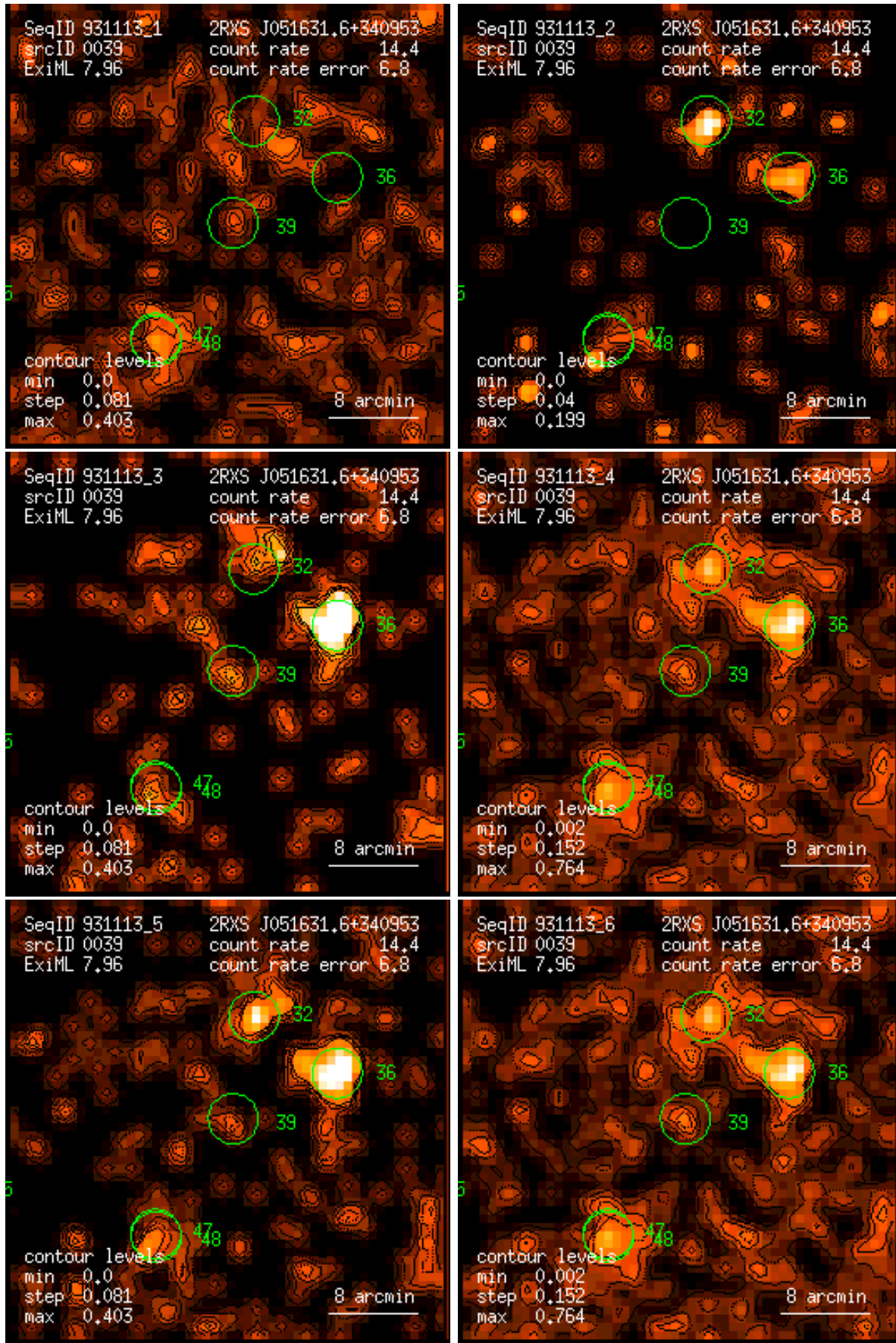
Figure 39: RASS 931113: detection 0039: band rate images, Gaussian filter: (1) PSPC channels 11 – 41, (2) 52 – 90, (3) 91 – 201, (4) 11 – 235, (5) 52 – 201, (6) 11 – 201. Broad band rates in counts/ks. Band rate contour levels in counts/ks/arcmin 2 .
