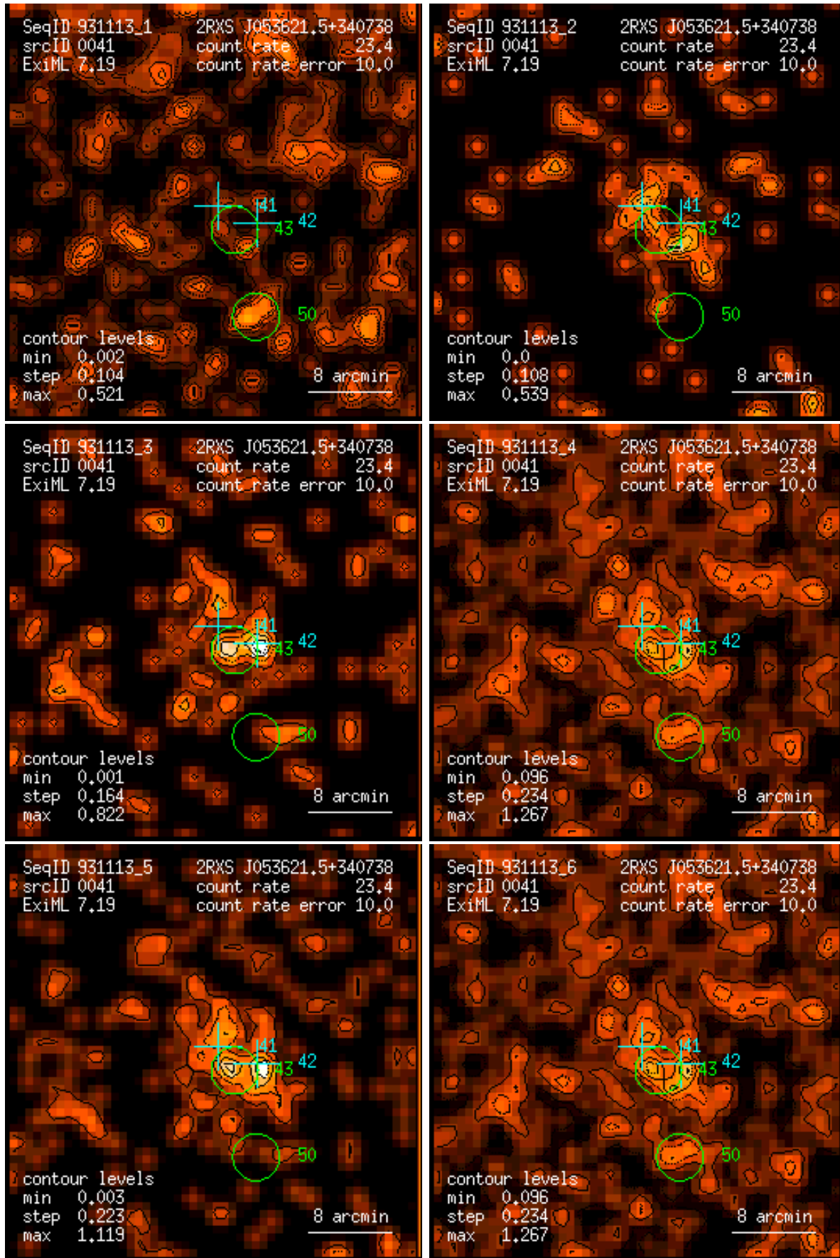
Figure 41: RASS 931113: detection 0041: band rate images, Gaussian filter: (1) PSPC channels 11 – 41, (2) 52 – 90, (3) 91 – 201, (4) 11 – 235, (5) 52 – 201, (6) 11 – 201. Broad band rates in counts/ks. Band rate contour levels in counts/ks/arcmin 2 .
