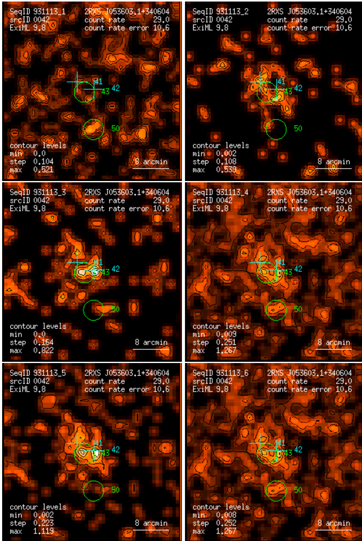
Figure 42: RASS 931113: detection 0042: band rate images, Gaussian filter: (1) PSPC channels 11 – 41, (2) 52 – 90, (3) 91 – 201, (4) 11 – 235, (5) 52 – 201, (6) 11 – 201. Broad band rates in counts/ks. Band rate contour levels in counts/ks/arcmin 2 .
